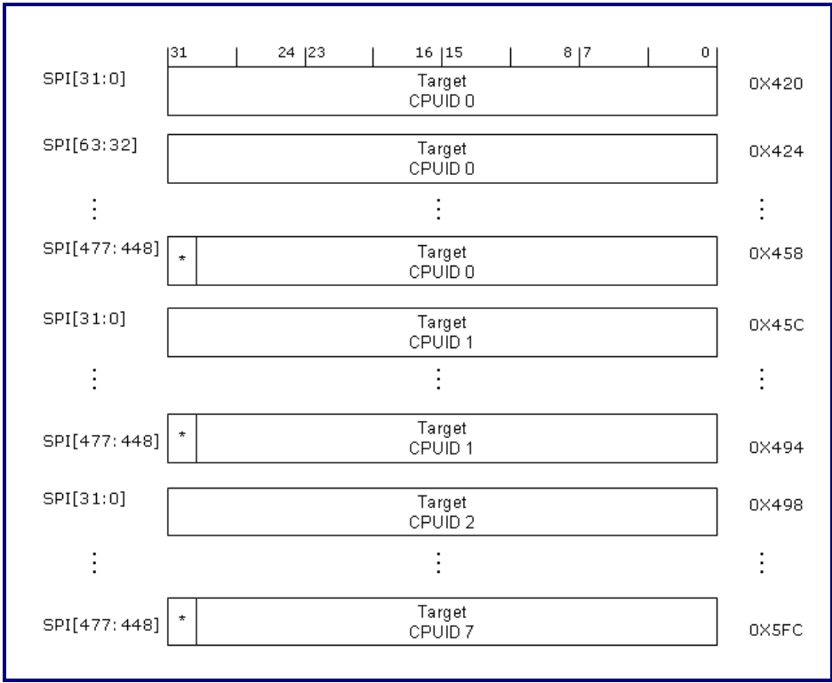
Figure 4-14. Base Address Offset of SPI Target Register
