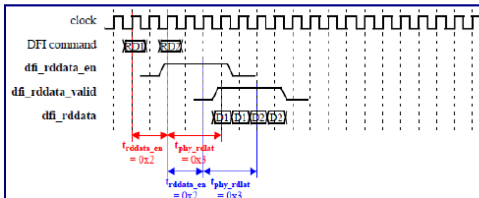
Figure 6-2. trddata_en and tphy_rdlat in DFI Specification 2.1
