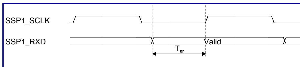
Figure 15-8. I 2 S Receiver Timing
