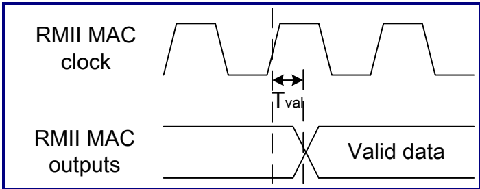
Figure 15-3. RMII MAC Output Timing
