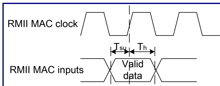
Figure 15-2. RMII MAC Input Timing
