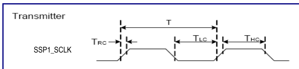
Figure 15-6. I 2 S Clock Timing
