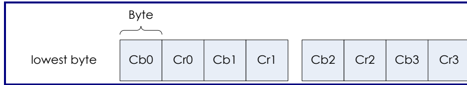
Figure 11-10. Semi-Planar Format of De-interleaved Chrominance
