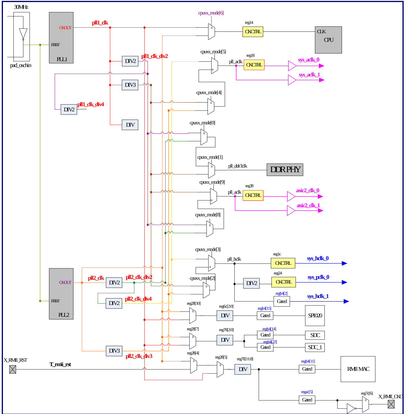
Figure 4-1. SCU Block Diagram for PLL1 and PLL2
