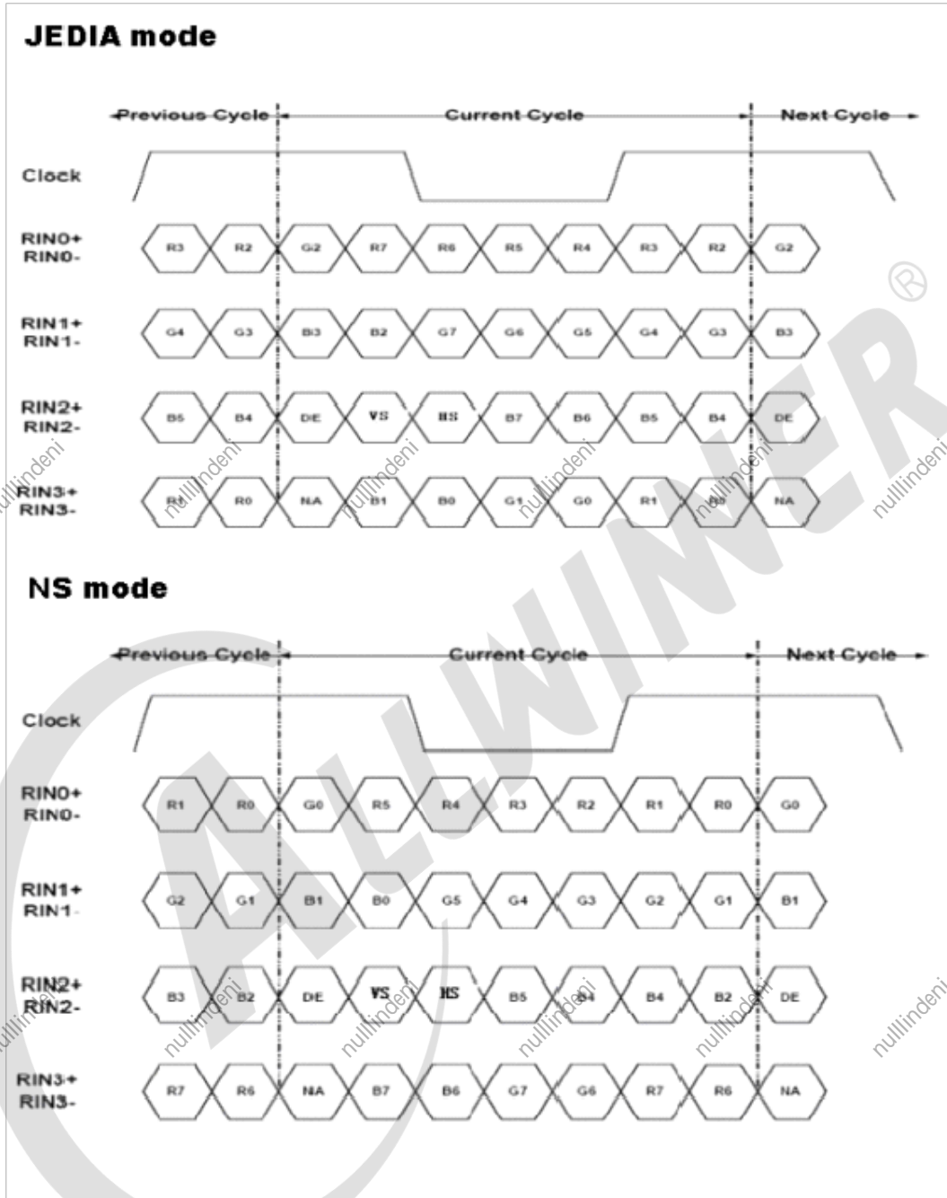
图 3: LVDS JEDIA mode and NS mode
