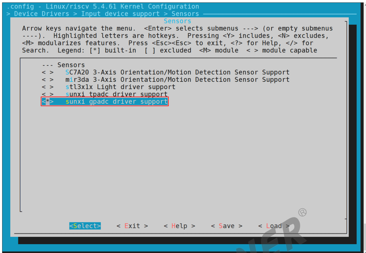
图 2-10: Device Drivers
