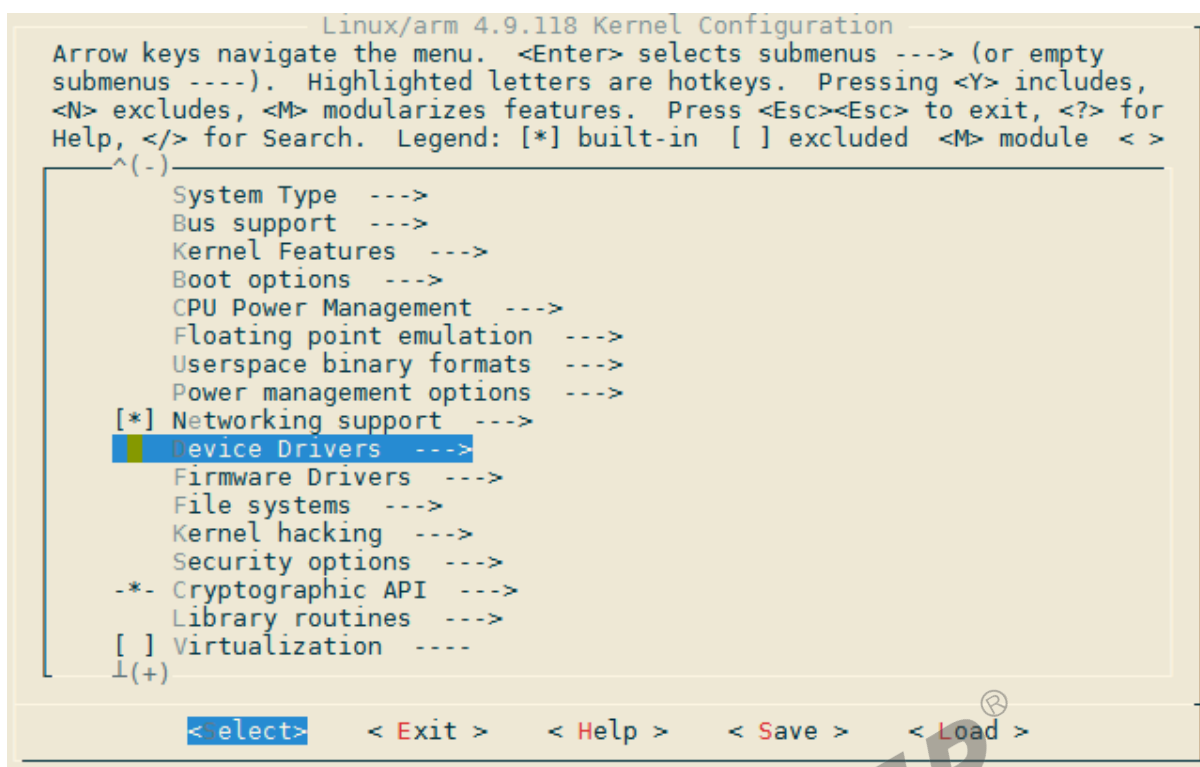
图 2-3: Device Drivers
