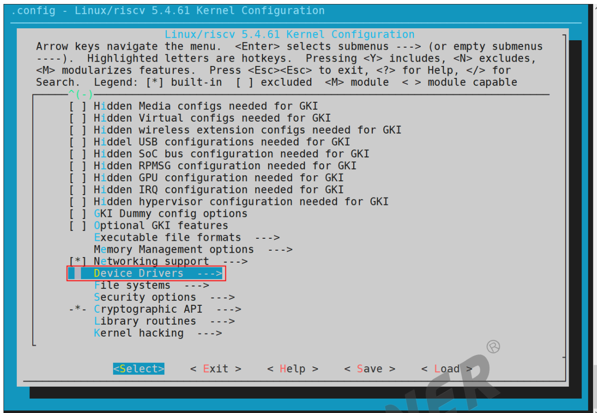
图 2-8: Device Drivers
