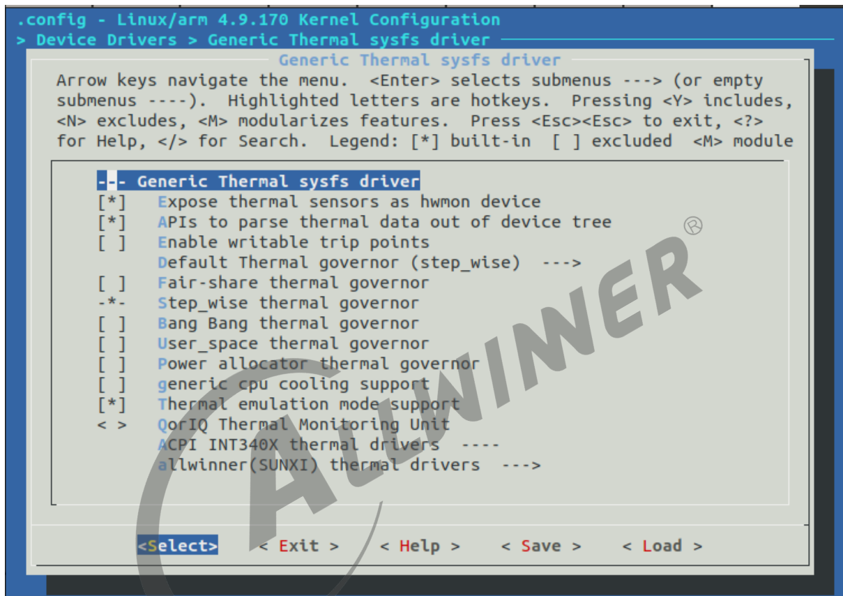
图 5-2: Thermal_menuconfig_R328_001.png
