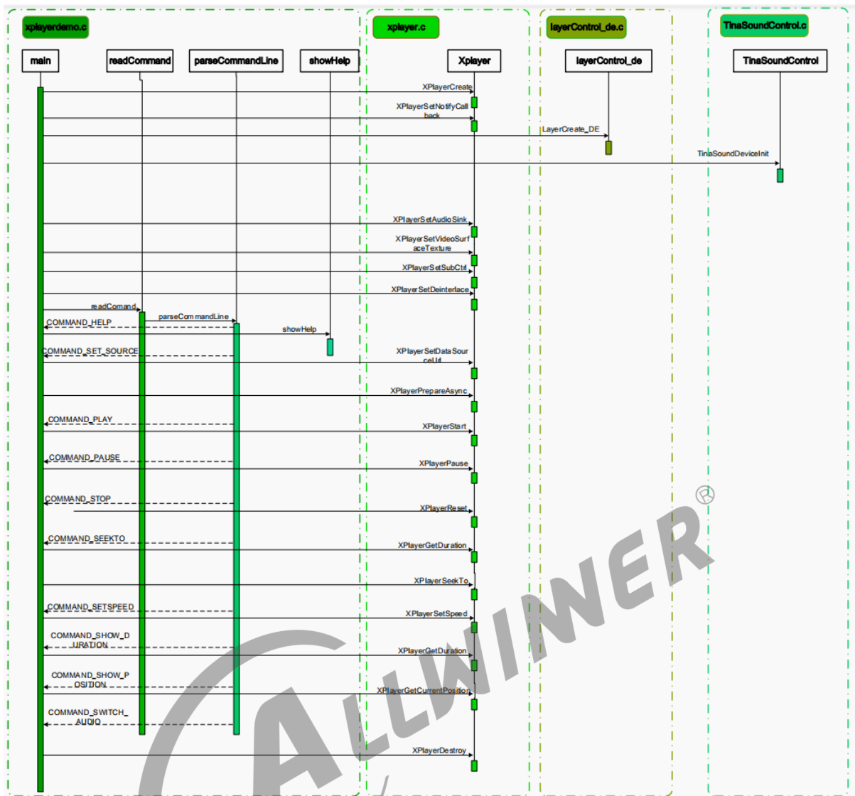
图 5-2: xplayerdemo 流程图
