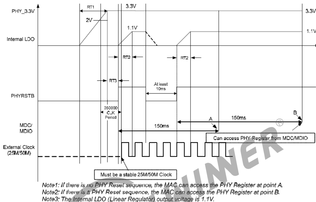
Figure 20. Power On and PHY Reset Sequence
