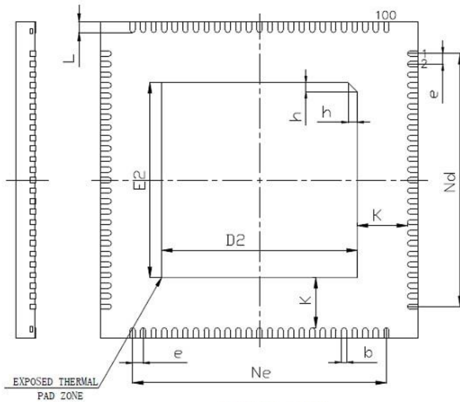
BOTTOM VIEW
