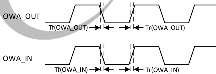
Figure 5-24 OWA Timing
