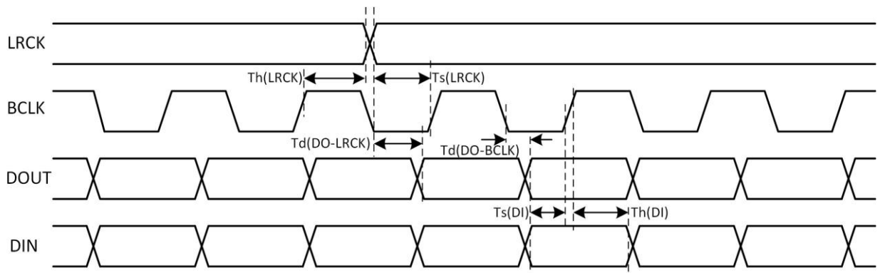
Figure 5-22 I2S/PCM Timing in Slave Mode
