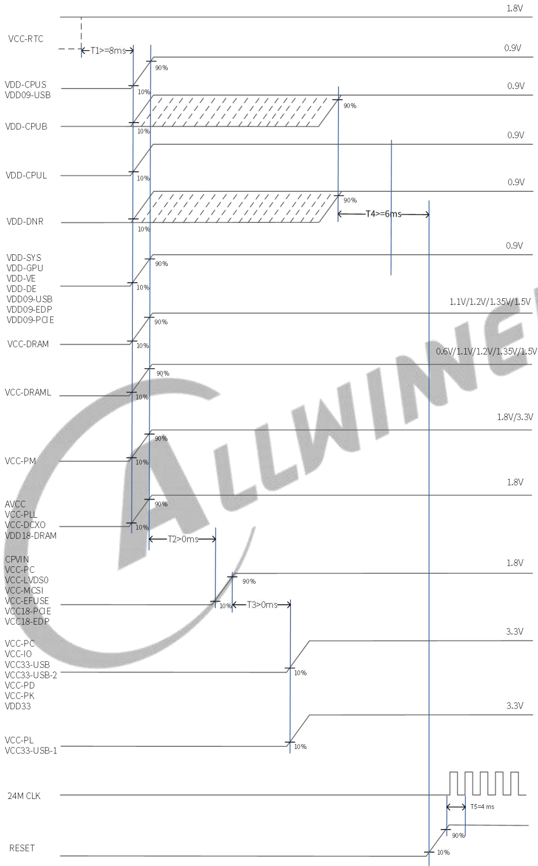
Figure 6-39 Power-on Timing
