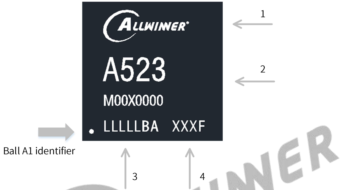
Figure 12-2 A523M00X0000 Marking
