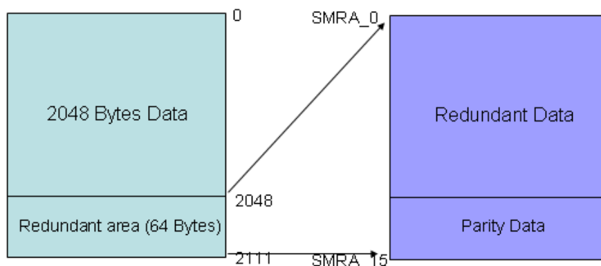
1.3.4-a Data arrangement for 2k page size and BCH algorithm
