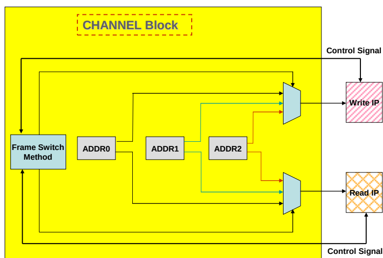
Figure 6.9-1 FSC Controller Block Diagram
