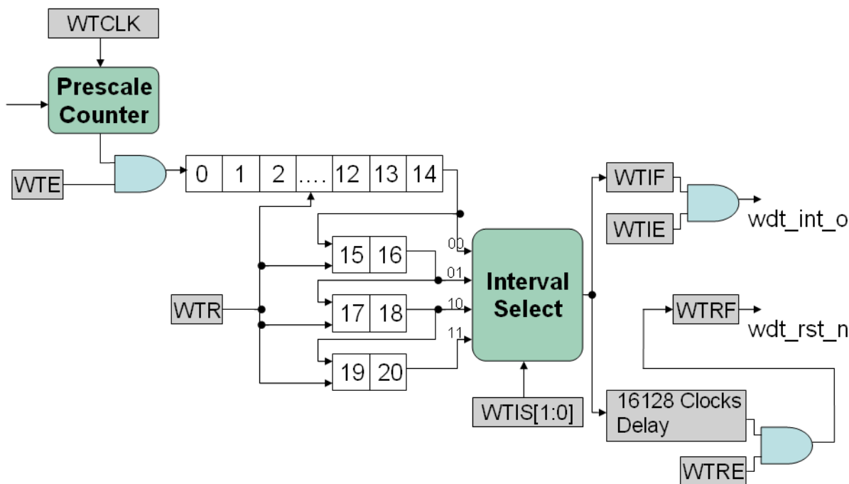
Figure 6.18-2 Watchdog Timer Block Diagram
