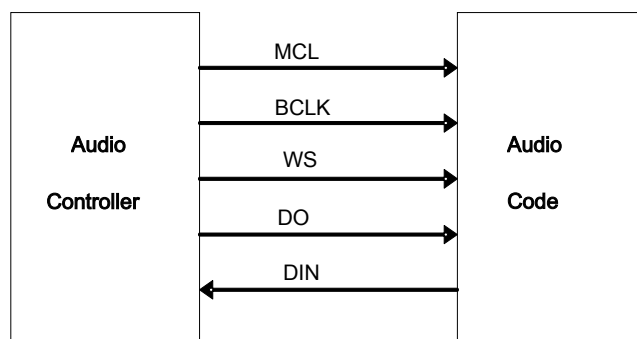
Figure 6.11.2 The interface signal of I2S
