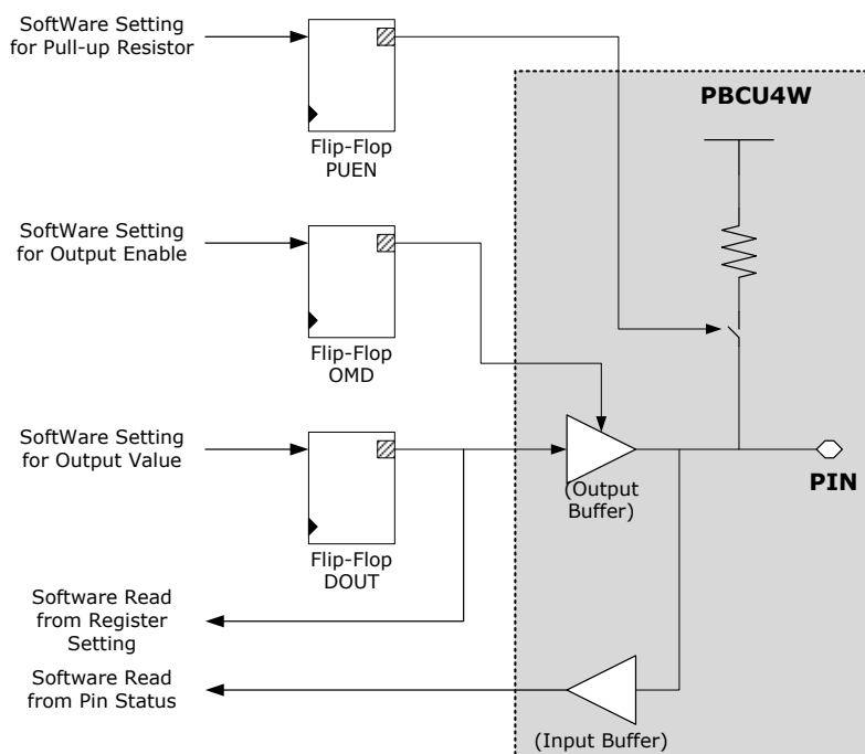
Figure 6.17-1 Type I GPIO: Input/Output Port with Program Controlled Weakly Pull-High
