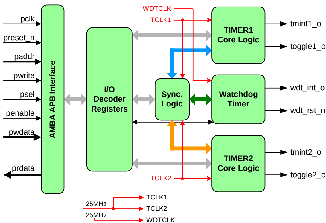
Figure 6.18-1 TIMER Block Diagram
