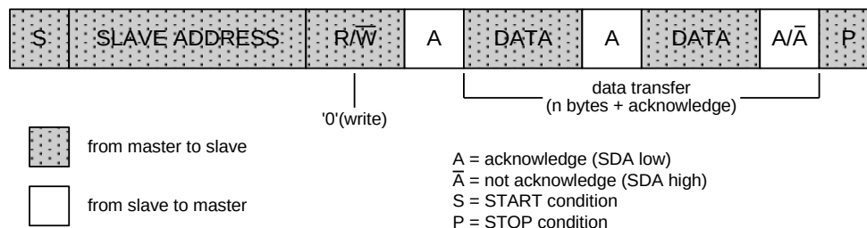
Data transfer on the I 2 C-bus
