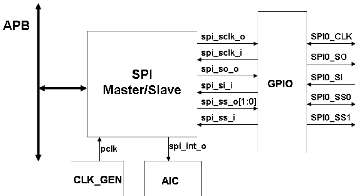
Figure 6.23-1 MICROWIRE/SPI Block Diagram (Master/Slave)
