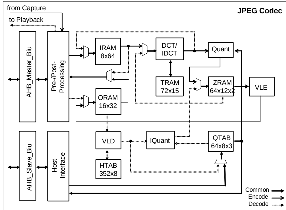
Figure 6.6-1 1 JPEG Codec block diagram
