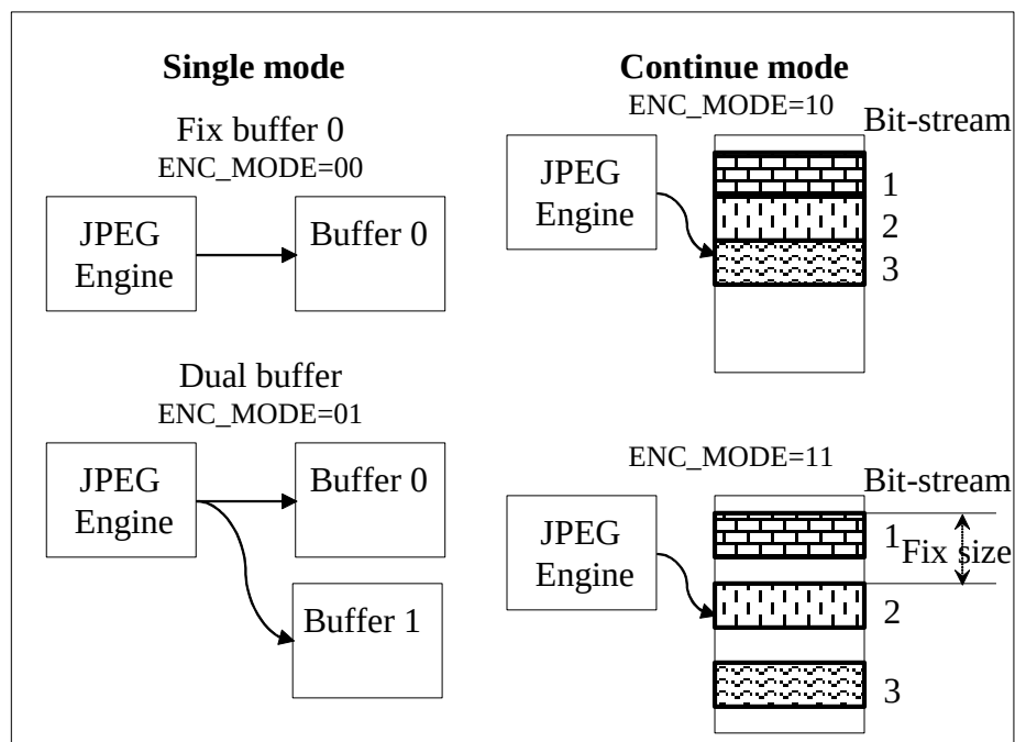
Figure 6.6-3. 4 Single mode and continue mode
