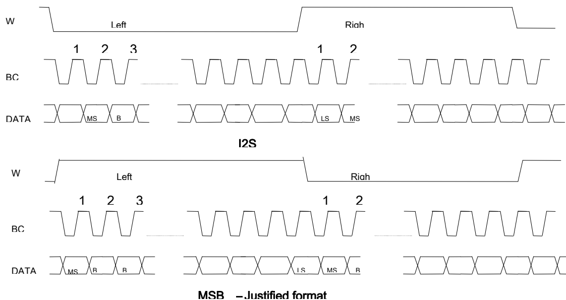
Figure 6.11.3 The format of I2S
