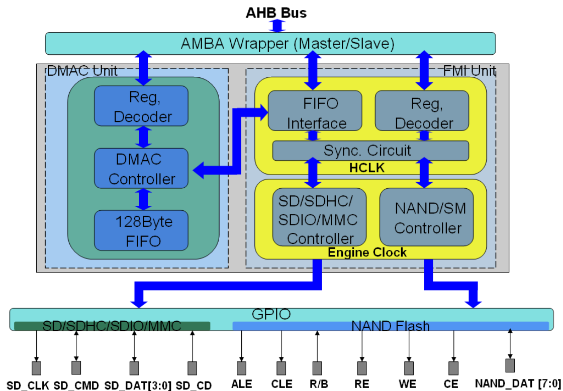
Figure 6.12-1 SIC Controller Block Diagram
