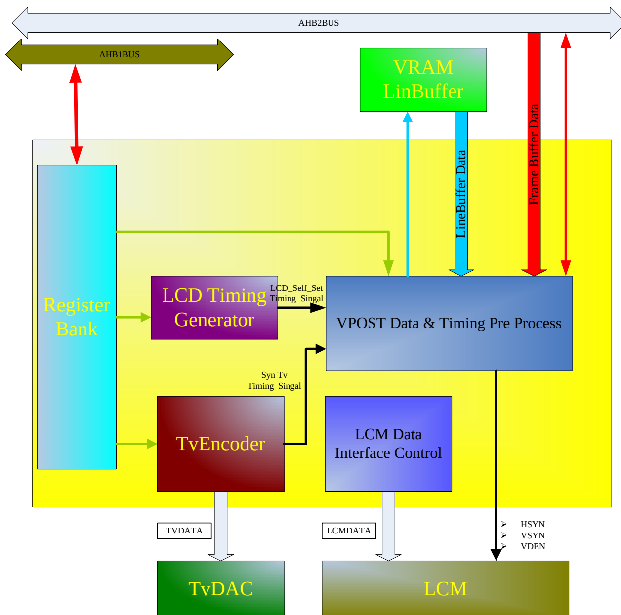
Figure 6.8-3 VPOST Controller Block Diagram
