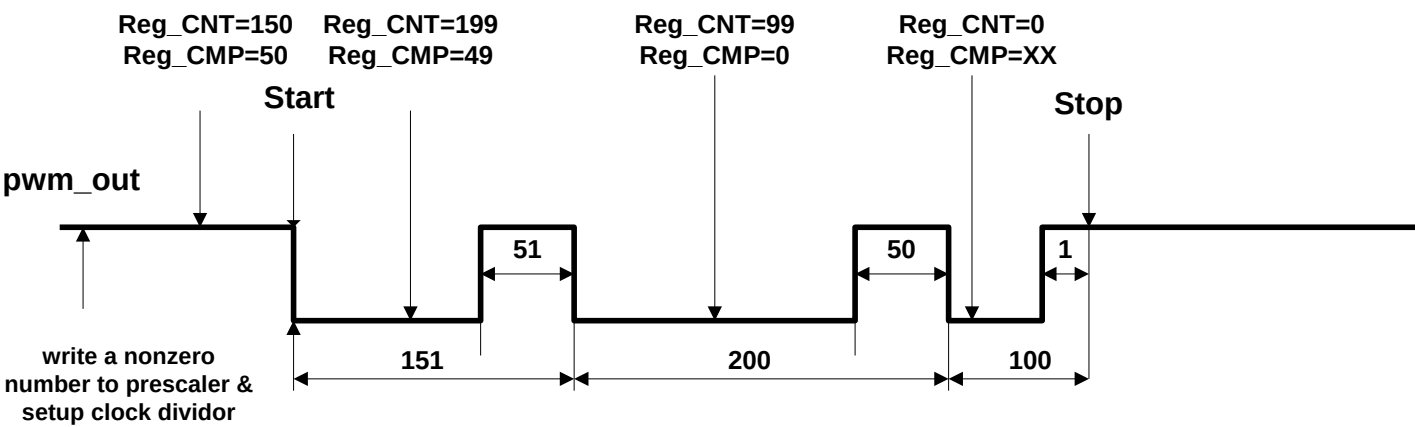
Figure 6.21-3 PWM Double Buffering Illustration
