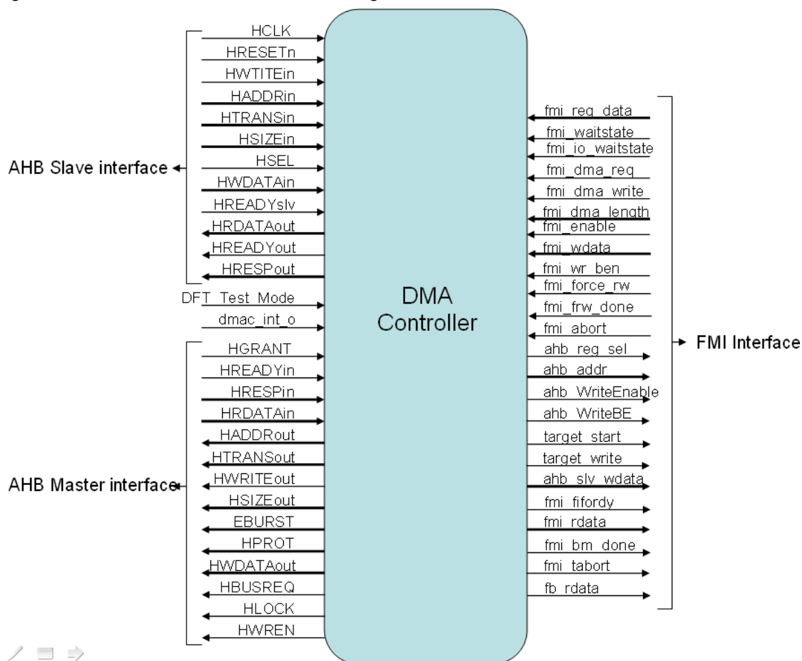
DMA Controller Symbol Diagram
