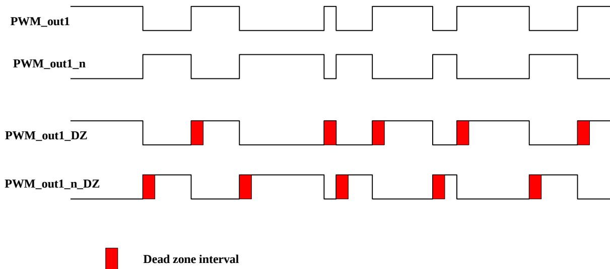
Figure 7.11-6.21-5 Dead Zone Generation Operation
