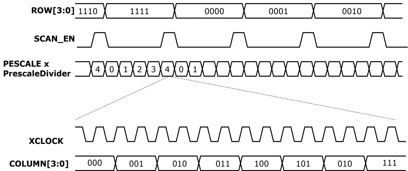
16x8 Keypad Scan Timing Diagram
