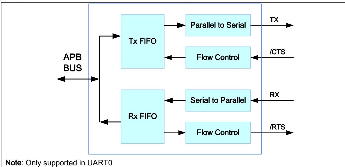
Auto Flow Control Block Diagram
