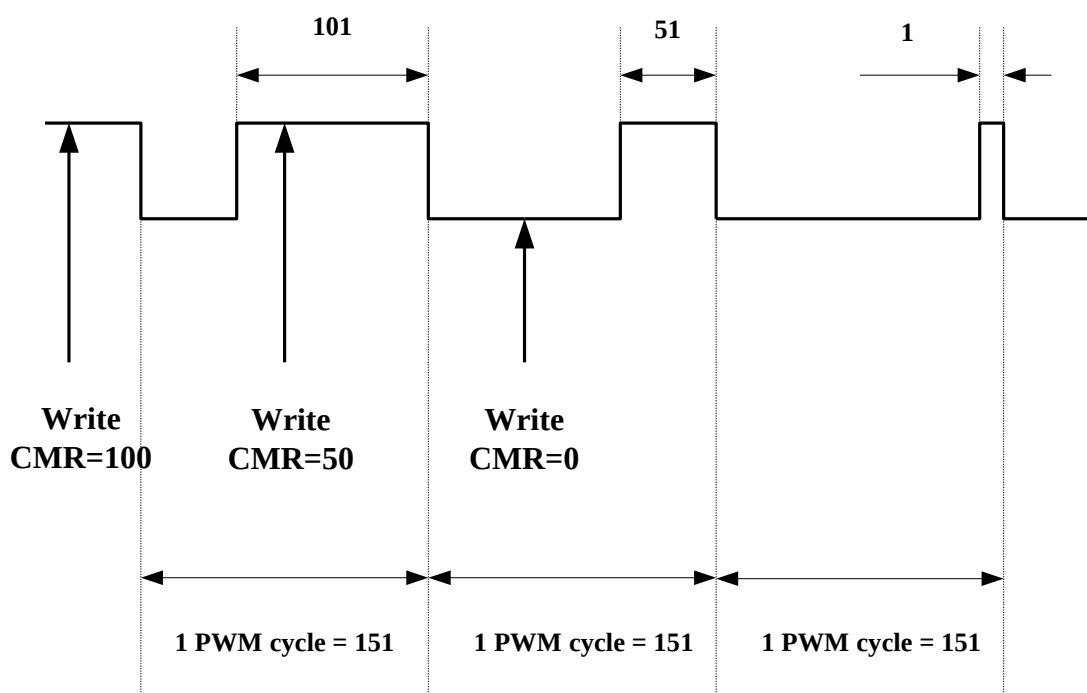
Figure 7.11-6.21-4 PWM Controller Output Duty Ratio
