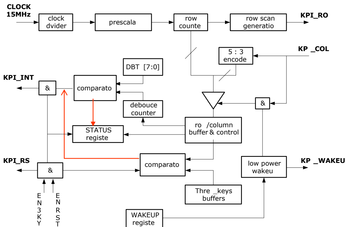
Keypad Controller Block Diagram
