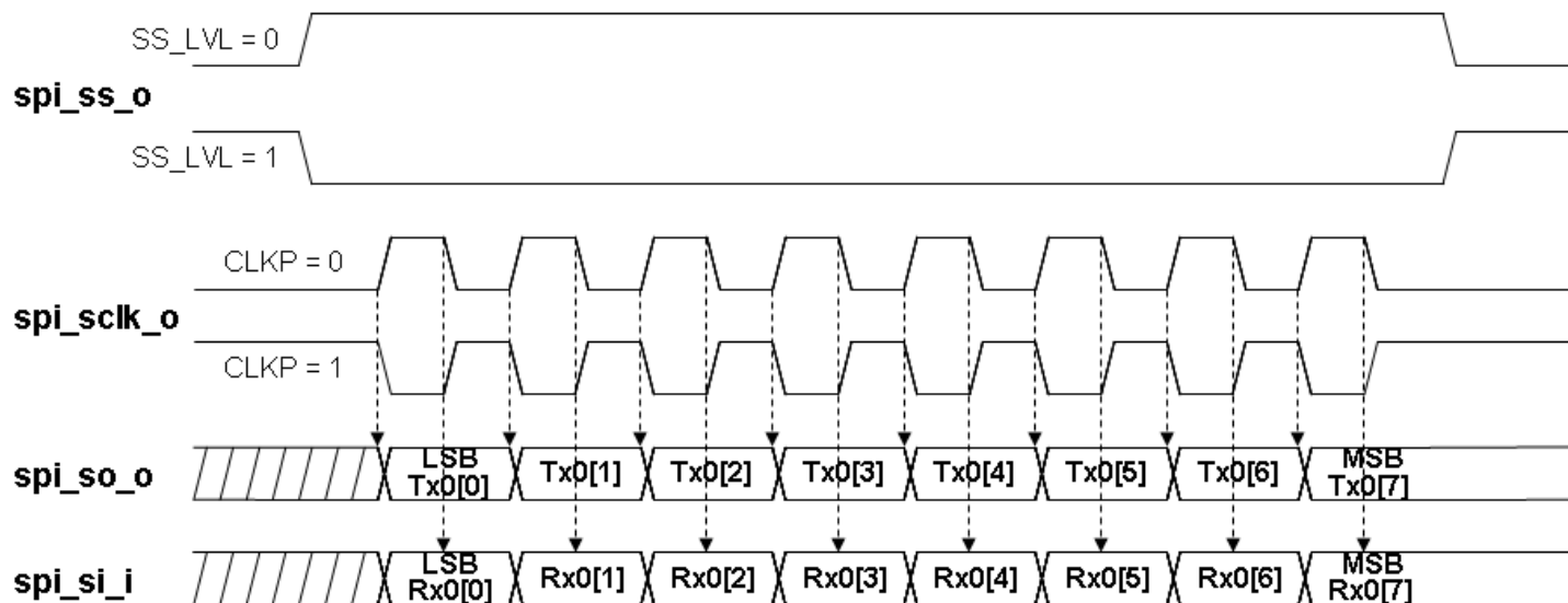
Figure 6.23-2 MICROWIRE/SPI Timing (Master)
