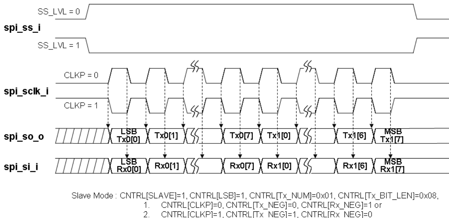
Figure 6.23-5 Alternate Phase SCLK Clock Timing (Slave)
