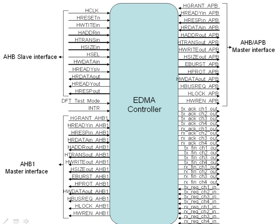
EDMA Controller Symbol Diagram
