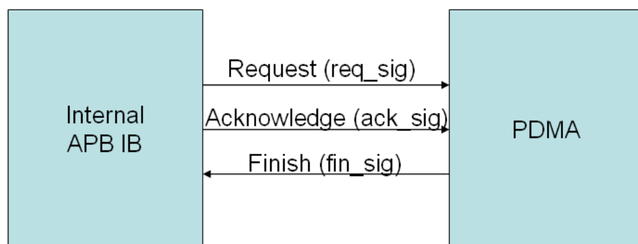
Figure 6.15-1 Peripheral interface signal
