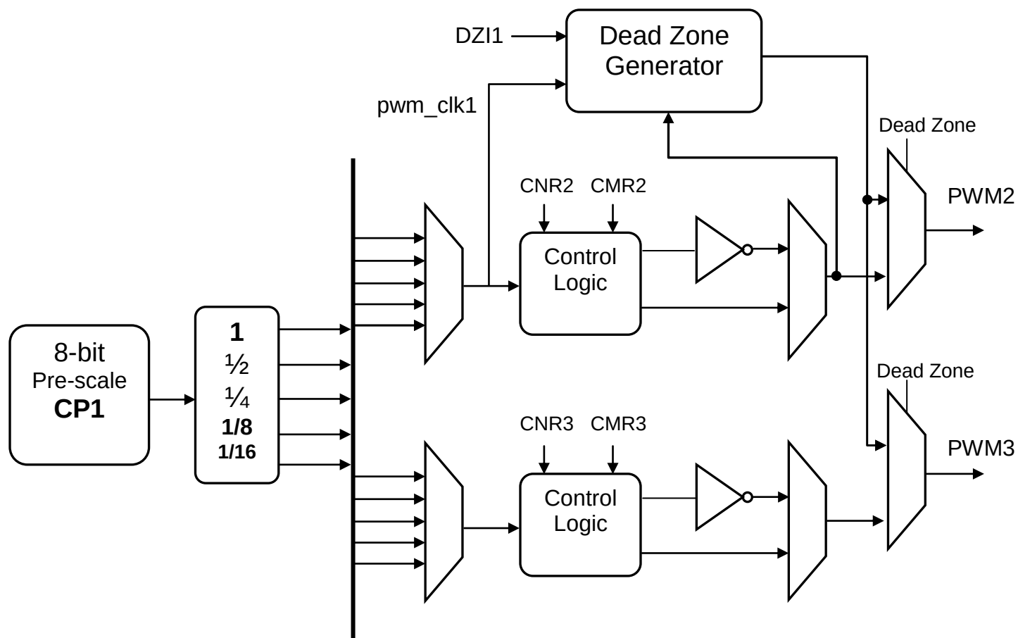
Figure 6.21-1 PWM Architecture Diagram
