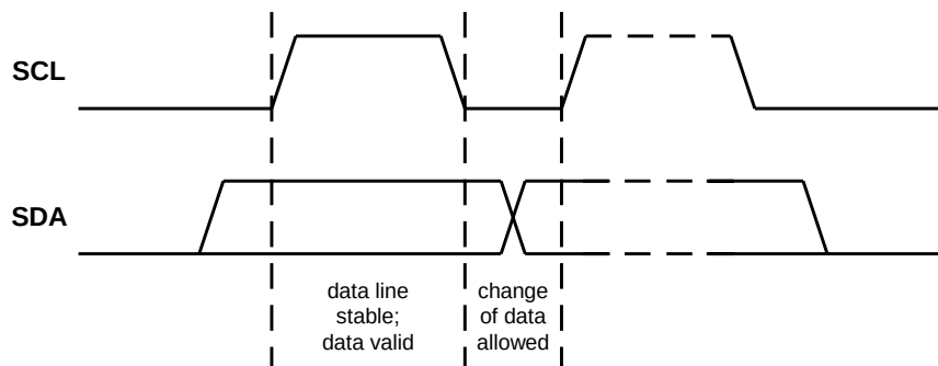
Bit transfer on the I 2 C-bus
