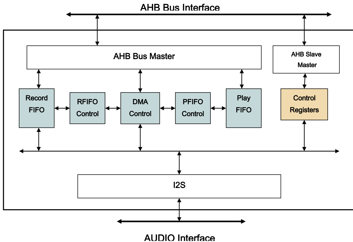
Figure 6.11.1 Block diagram of Audio Controller
