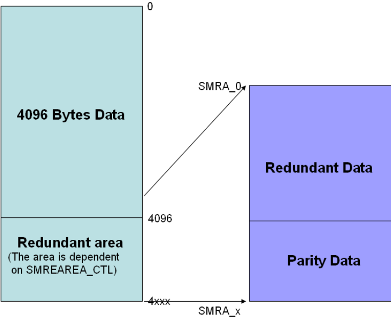
1.3.4-b Data arrangement for 4k page size NAND flash
