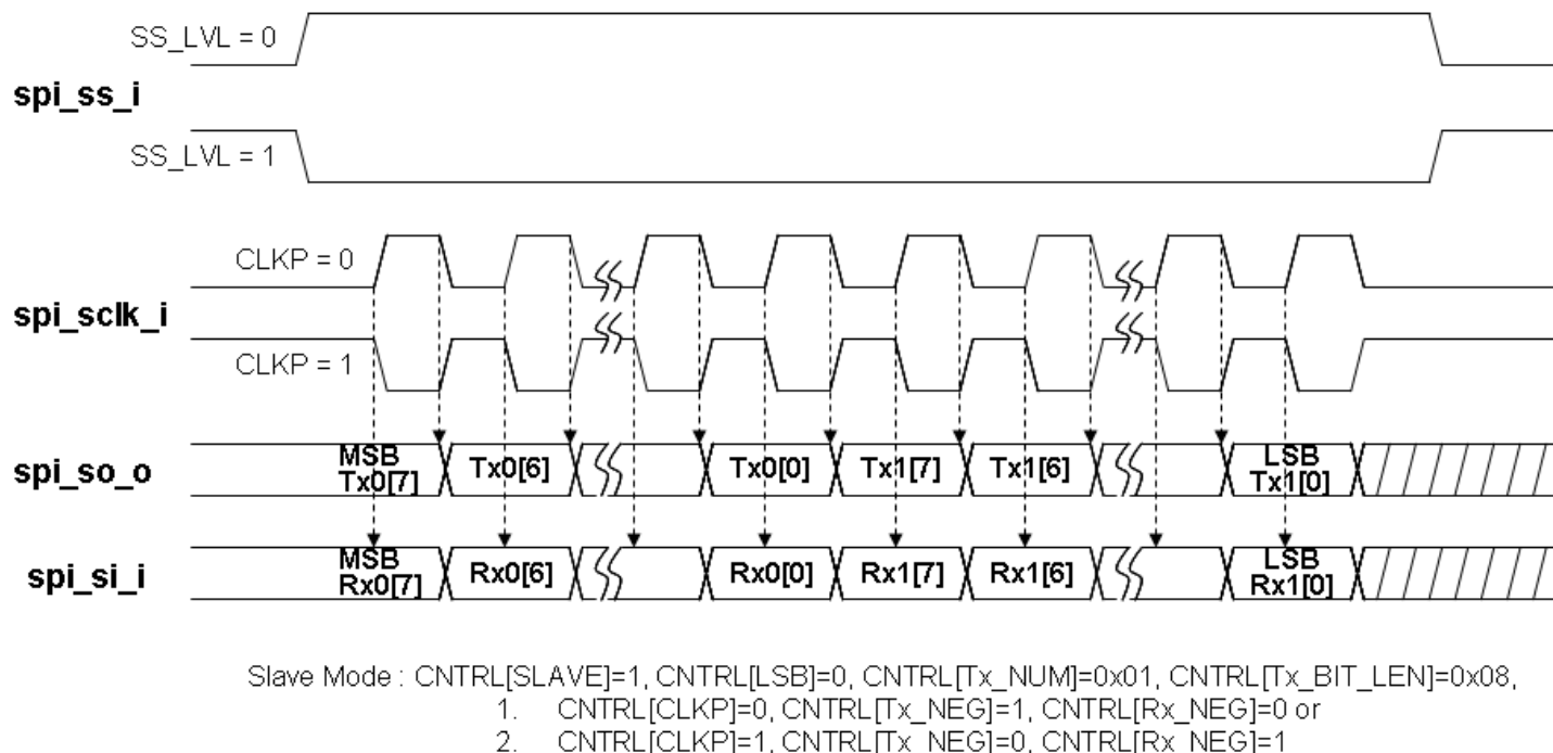
Figure 6.23-4 MICROWIRE/SPI Timing (Slave)
