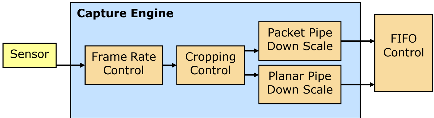
FIG-1 Functional Block Diagram
