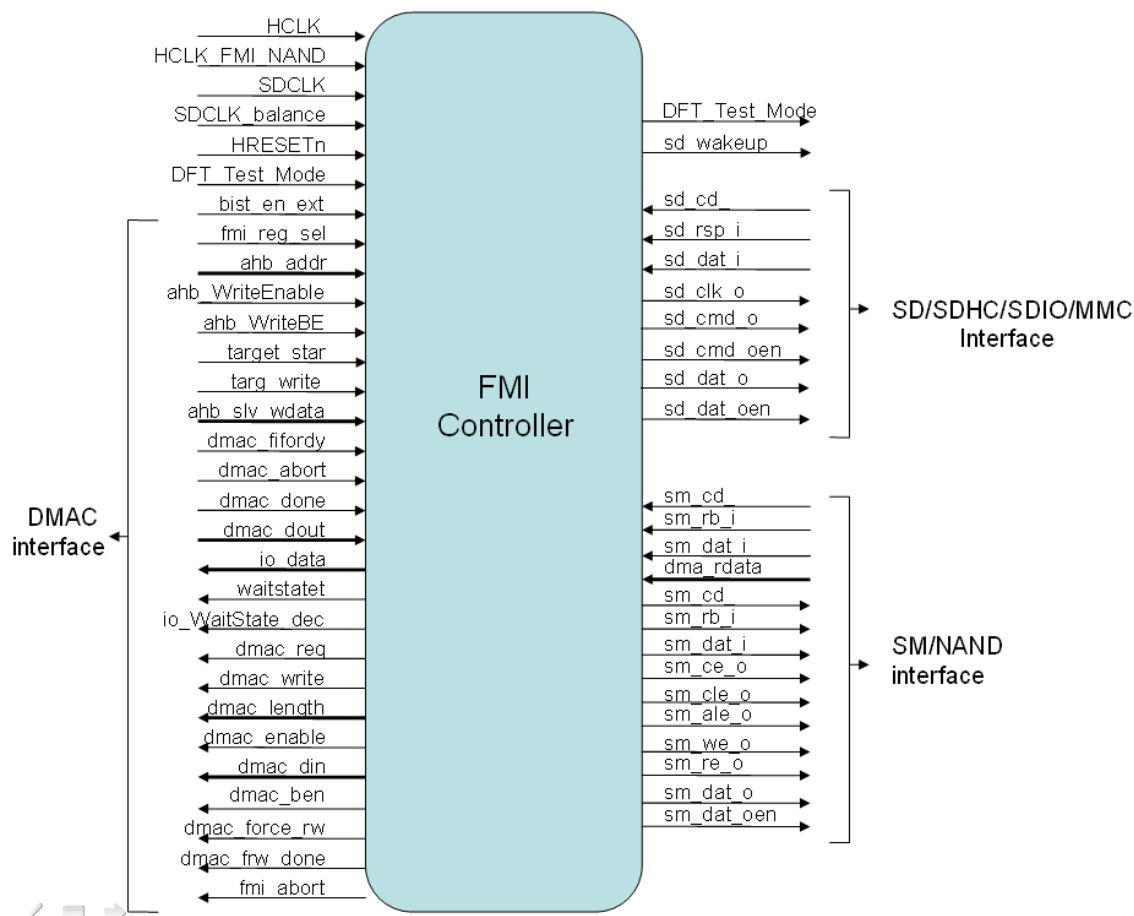
FMI Controller Symbol Diagram
