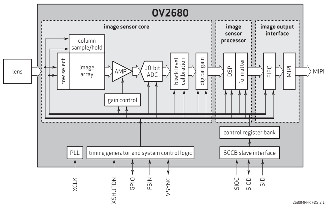
figure 2-1 OV2680 block diagram
