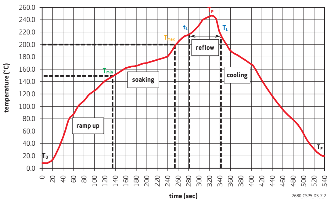
figure 7-2 IR reflow ramp rate requirements
