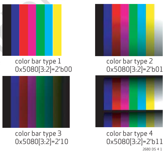
figure 4-1 color bar test patterns
