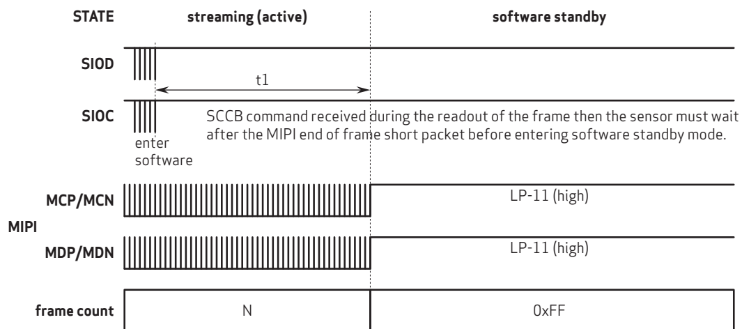
figure 6-2 standby sequence
