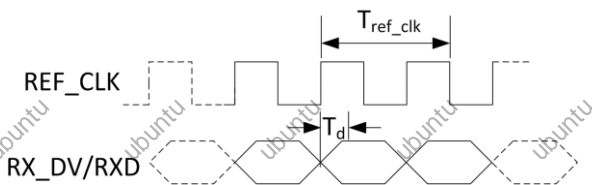
Figure 5-21 RMII Interface Receive Timing
