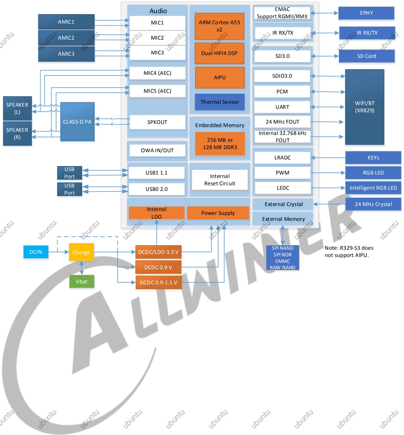
Figure 3-2 R329 Intelligent Speaker Solution
