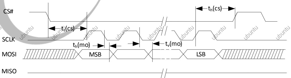
Figure 5-22 SPI Writing Timing
