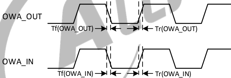
Figure 5-31 OWA Timing
