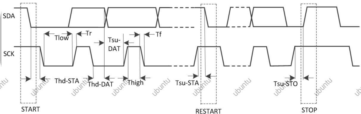
Figure 5-27 TWI Timing
