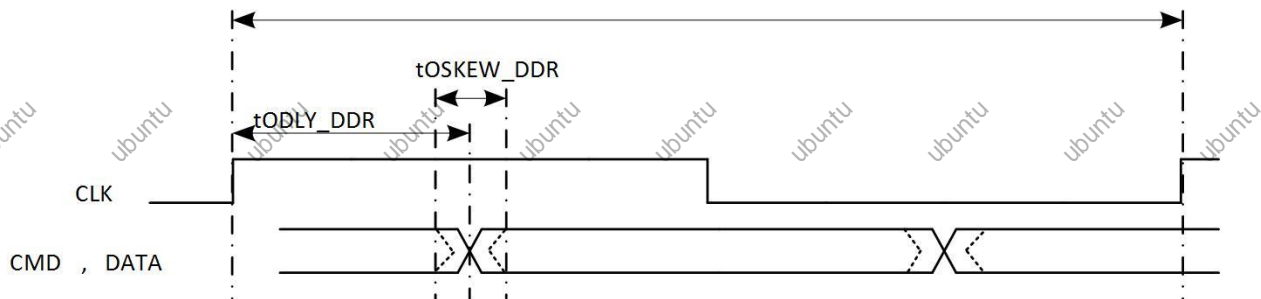
Figure 5-14 SMHC HS-DDR Mode Output Timing Diagram
