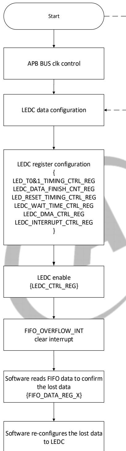
Figure 9-102 FIFO Overflow Abnormal Processing Flow
