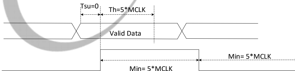
Figure 8-9 Timing Requirements for Inputs
