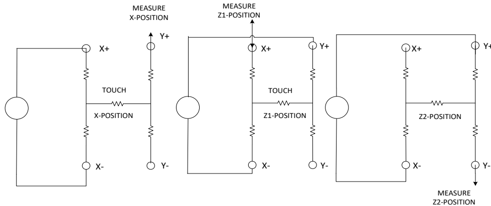
Figure 9-77 Touch Pressure Measurement for Touch Panel
