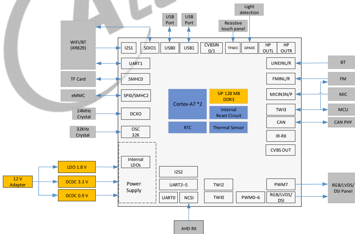
Figure 2-3 Car Instrument Solution of the T113-S3
