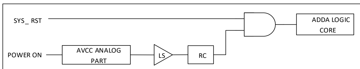
Figure 8-22 Audio Codec Analog Part Reset System
