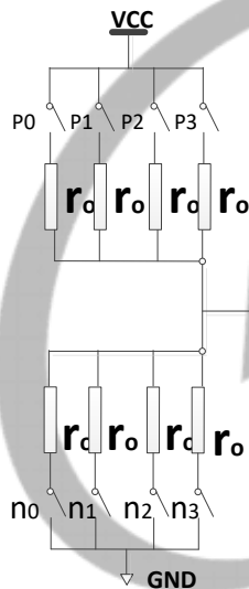
Figure 9-69 IO Buffer Strength Diagram
