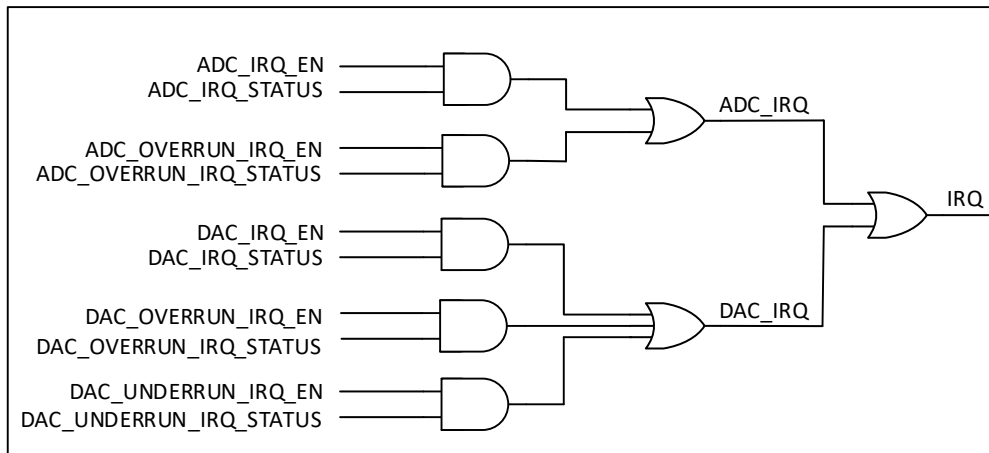
Figure 8-25 Audio Codec Interrupt System
