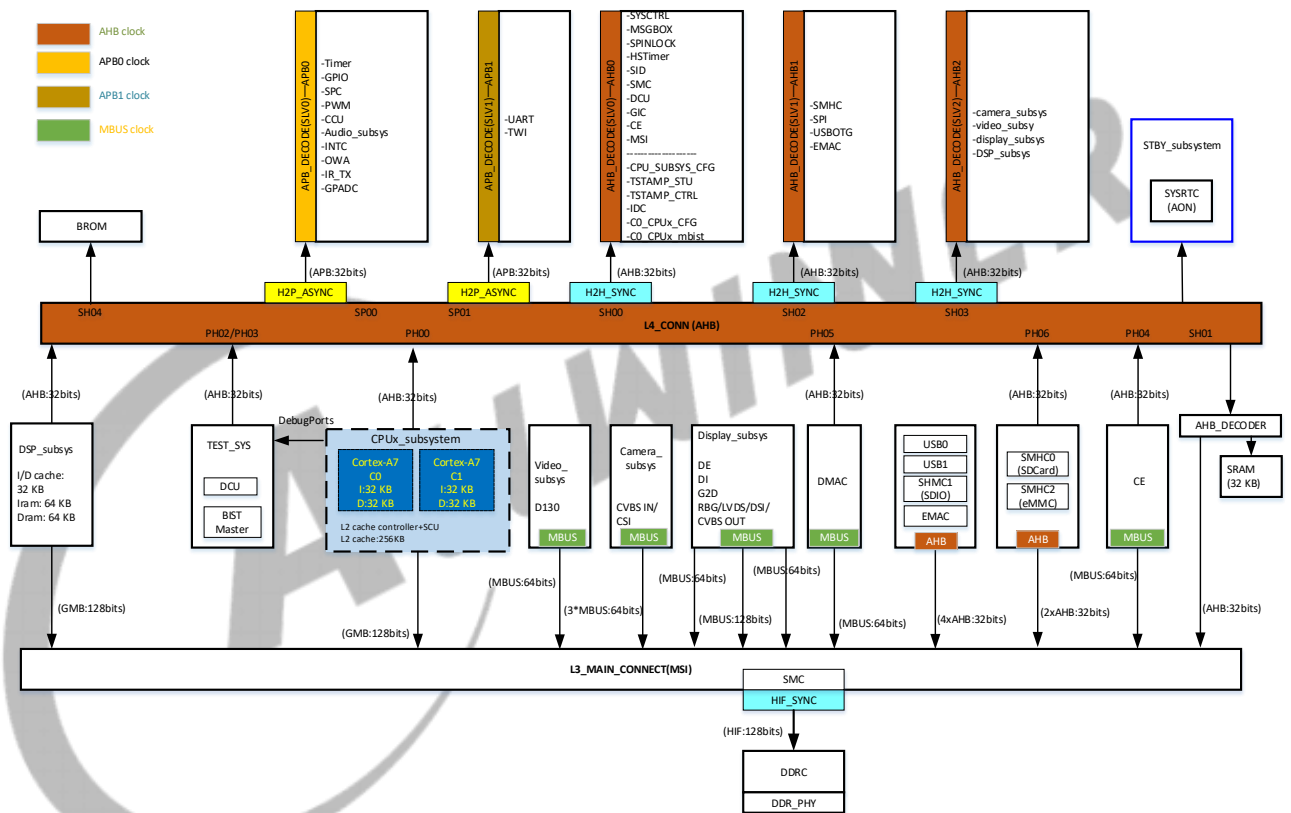
Figure 3-3 System Bus Tree
