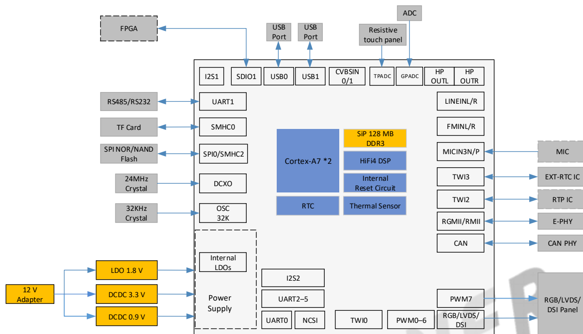
Figure 2-5 PLC Solution of the T113-S3
