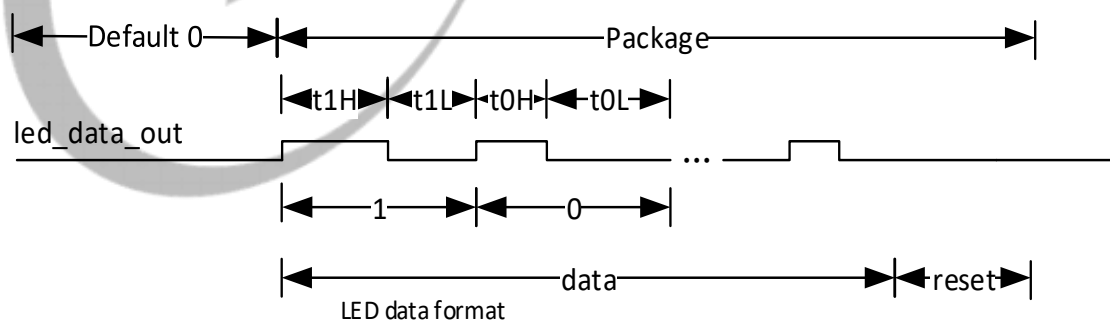
Figure 9-94 LEDC Package Output Timing Diagram
