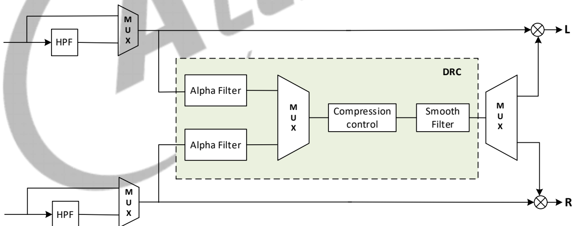
Figure 8-26 DAP Data Flow
