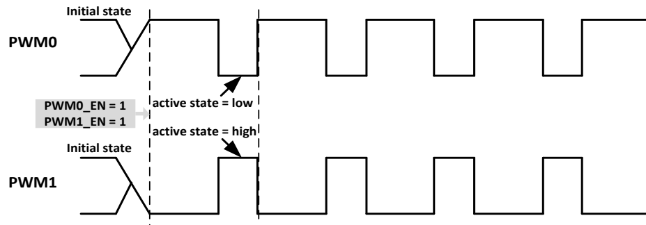
Figure 9-88 PWM01 Complementary Pair Output
