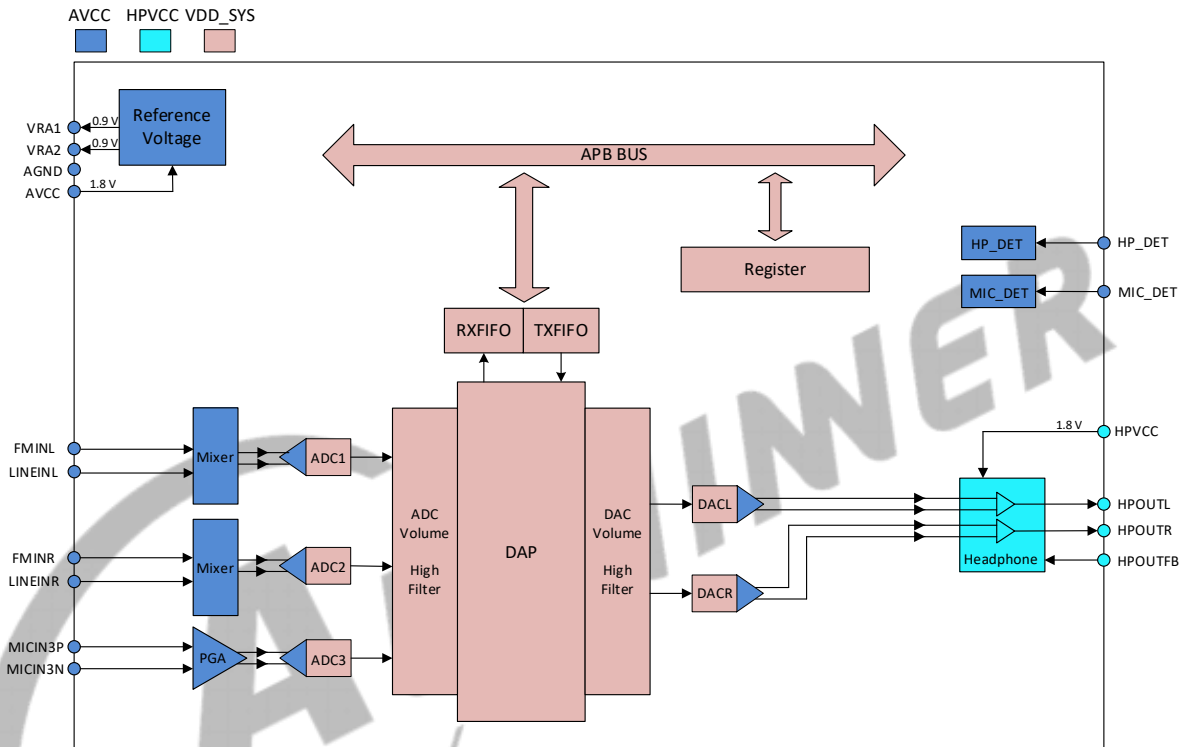
Figure 8-19 Audio Codec Block Diagram
