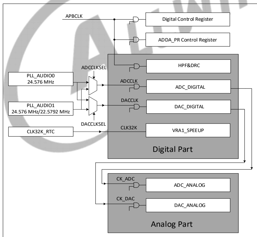
Figure 8-20 Audio Codec Clock Diagram
