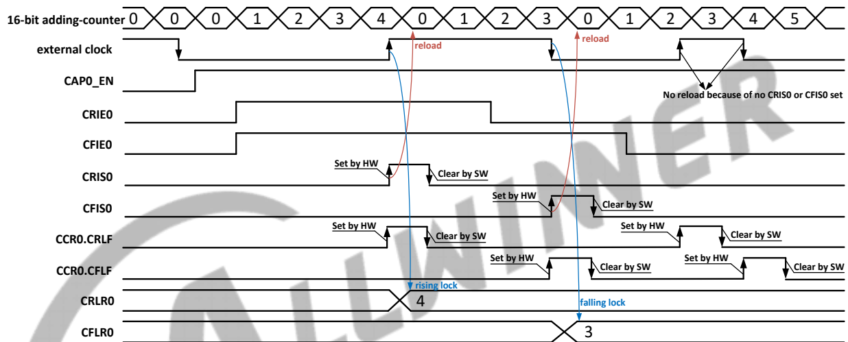
Figure 9-92 PWM0 Channel Capture Timing
