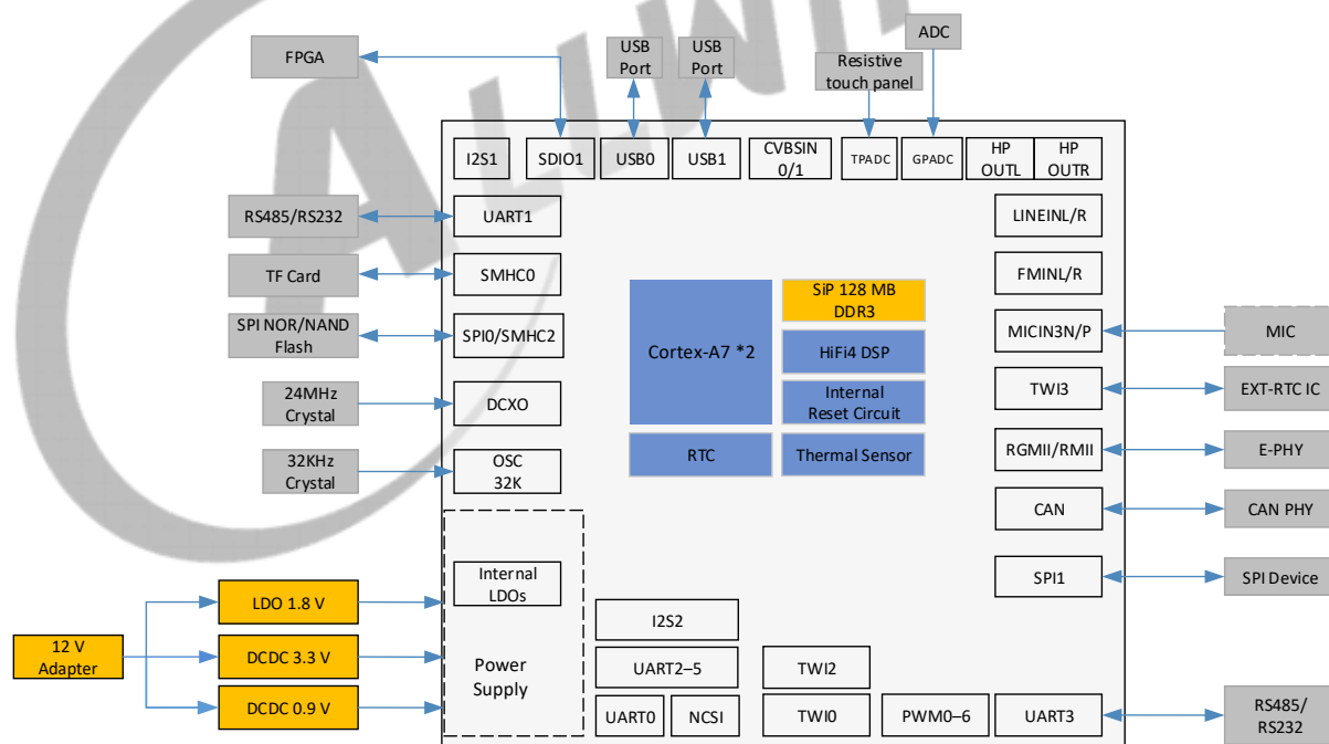
Figure 2-5 PLC Solution of the T113-S3
