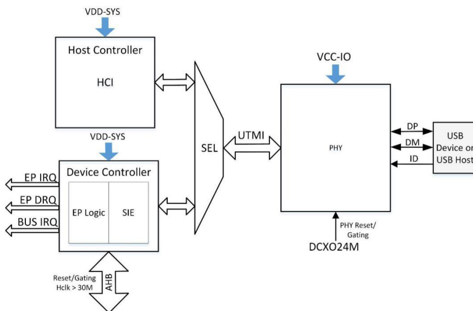
Figure 9-64 USB2.0 DRD Controller and PHY Connection Diagram
