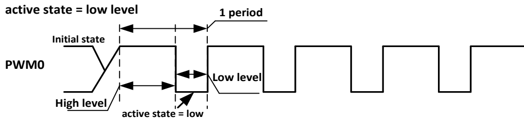
Figure 9-85 PWM0 Low Level Active State
