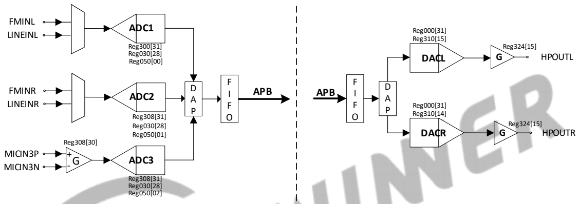
Figure 8-23 Audio Codec Data Path Diagram
