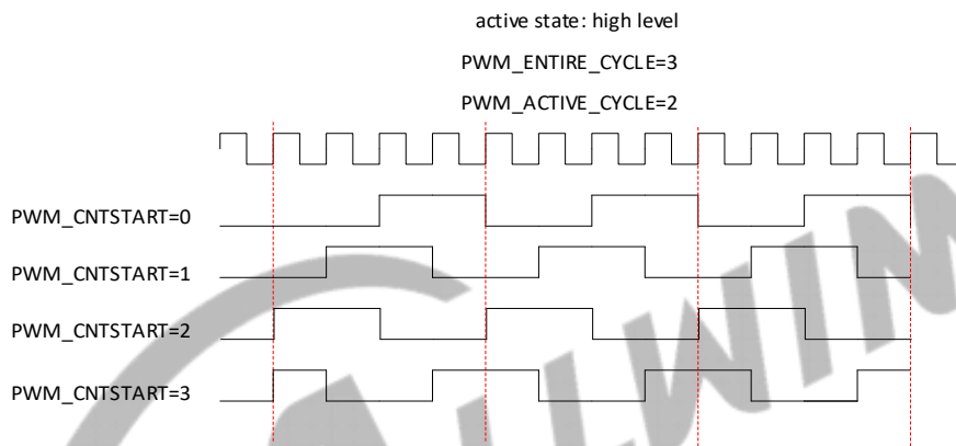
Figure 9-86 Phase of PWM0 High Level Active State
