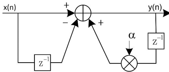
Figure 8-27 HPF Logic Structure
