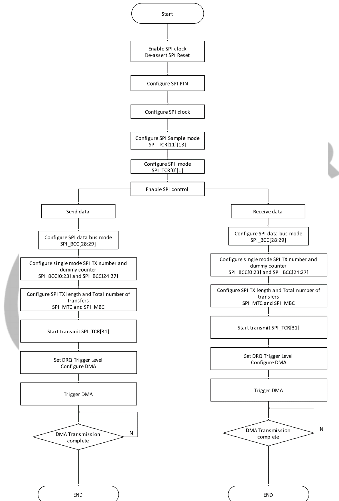
Figure 9-62 SPI Write/Read Data in DMA Mode
