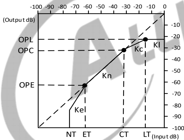
Figure 8-29 DRC Static Curve Parameters
