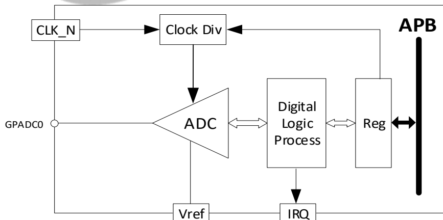
Figure 9-70 GPADC Block Diagram
