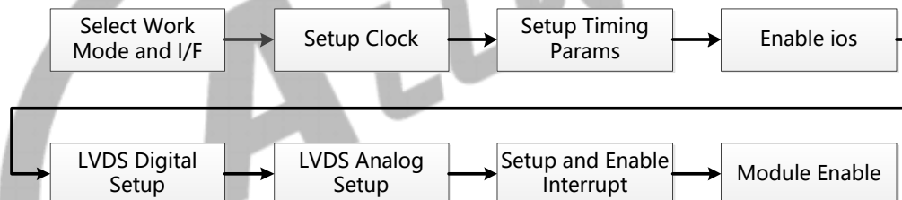
Figure 5-12 LVDS Mode Configuration Process
