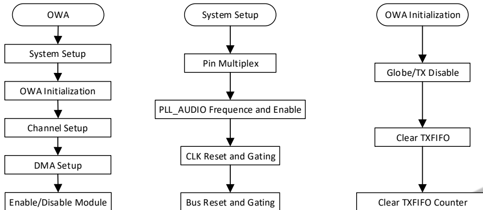
Figure 8-18 OWA Operation Flow
