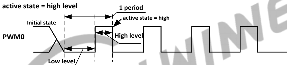
Figure 9-84 PWM0 High Level Active State
