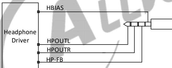
Figure 8-24 Headphone Output Application
