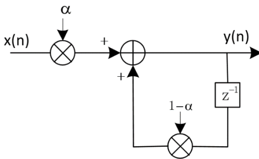
Figure 8-30 Energy Filter Structure
