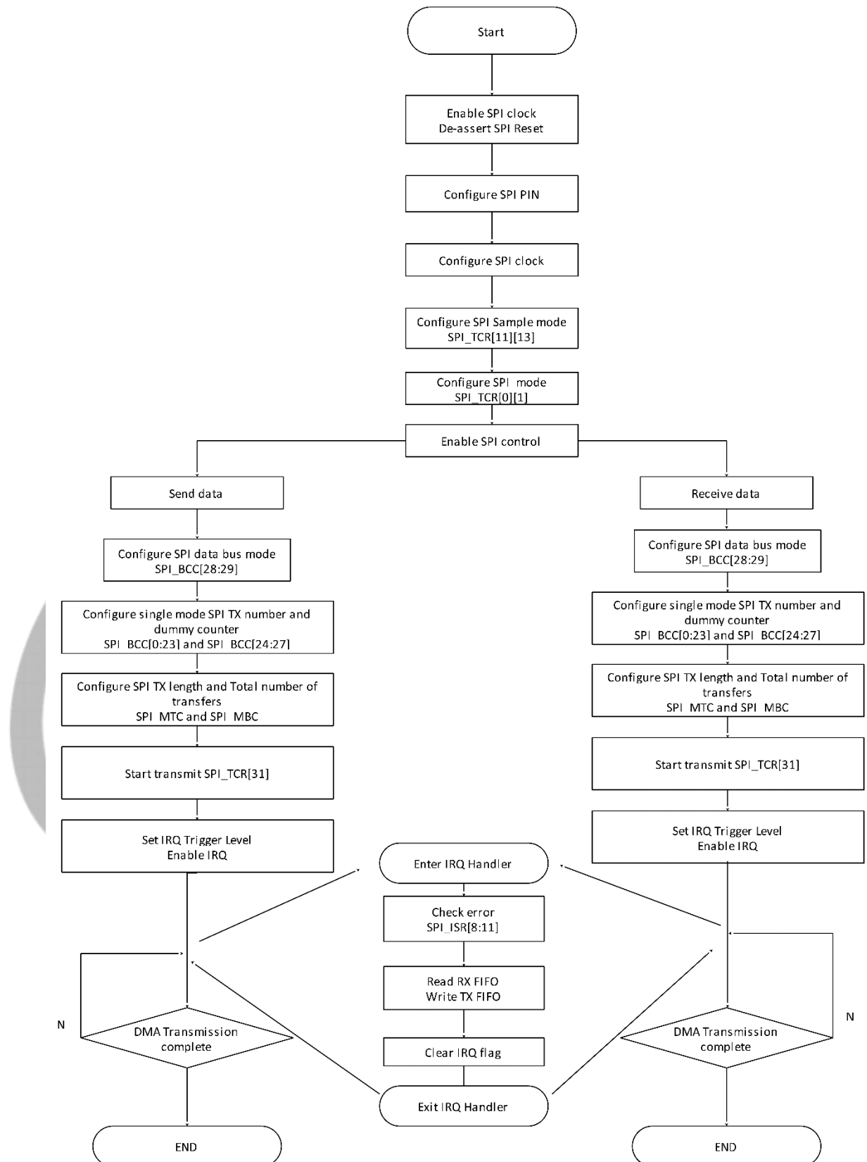
Figure 9-61 SPI Write/Read Data in CPU Mode
