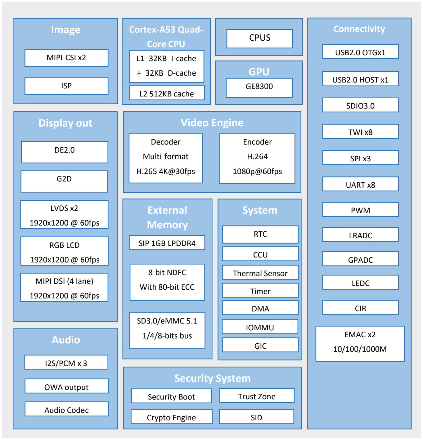
Figure 3-1. SW106 Block Diagram
