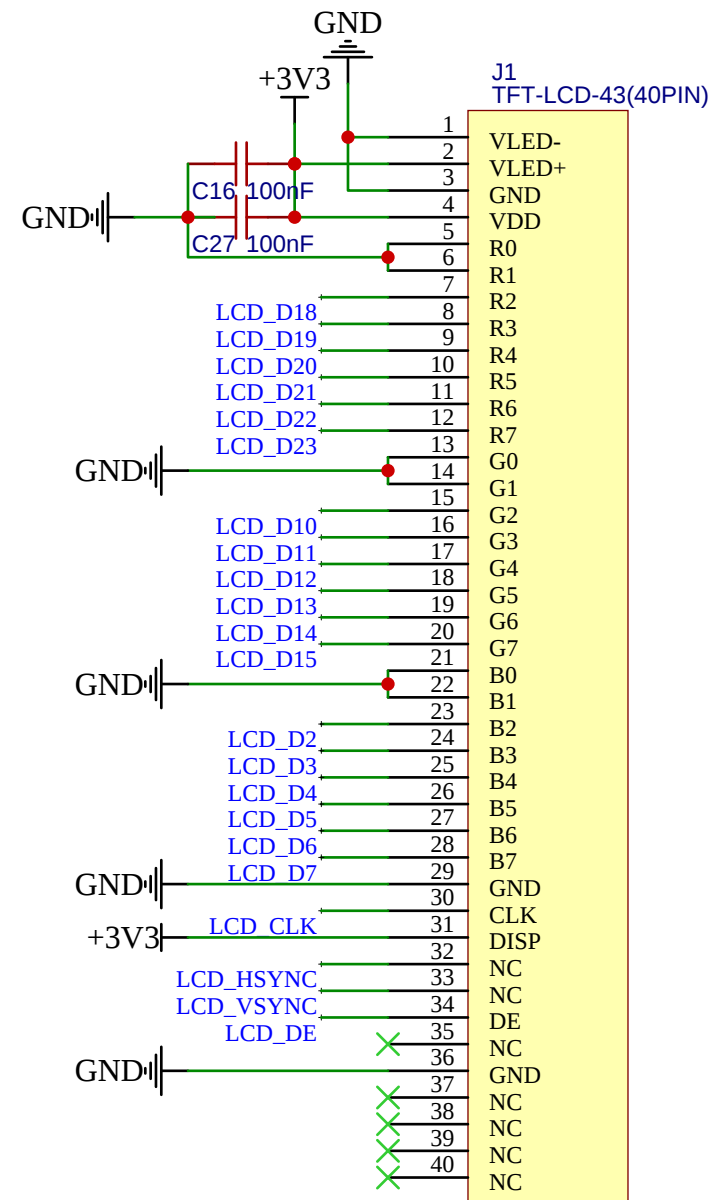
LCD/40pin/rgb
