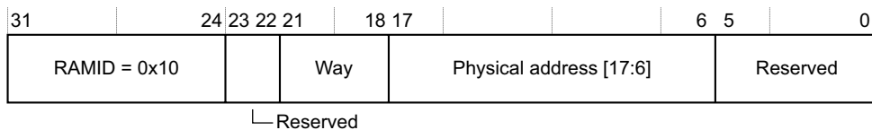
Figure 4-53 RAMINDEX bit assignments for L2 tag RAM
