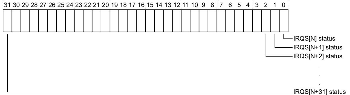
Figure 8-4 GICD_SPISR bit assignments
