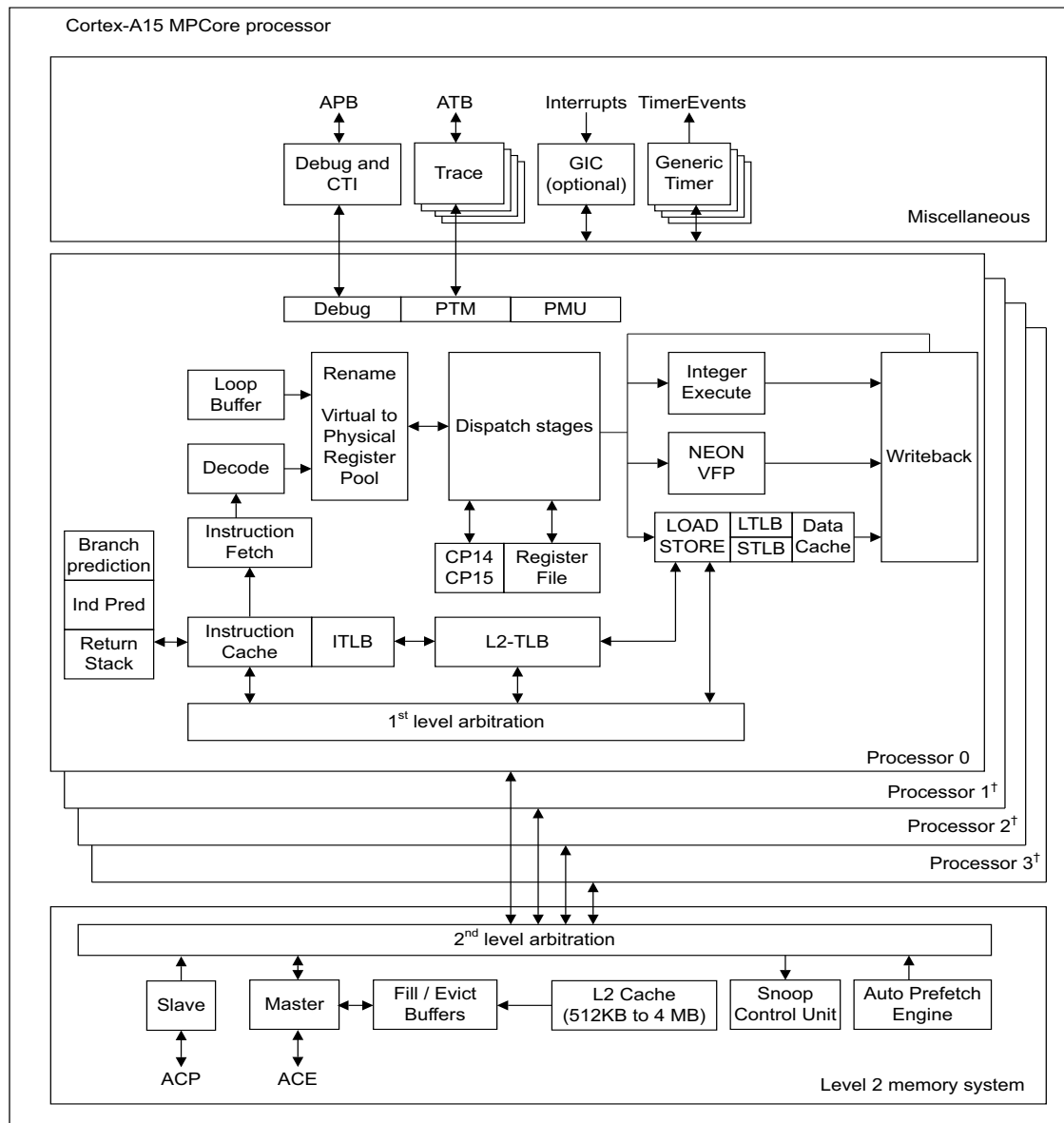
Figure 2-1 Block diagram
