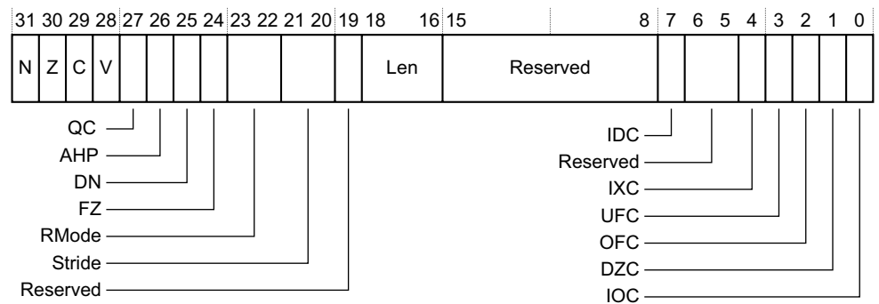
Figure 14-2 FPSCR bit assignments
