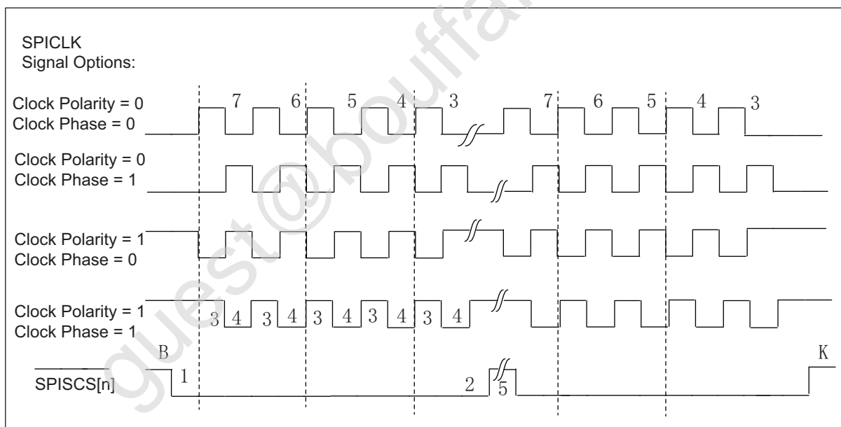
Fig. 9.1: SPI clock
