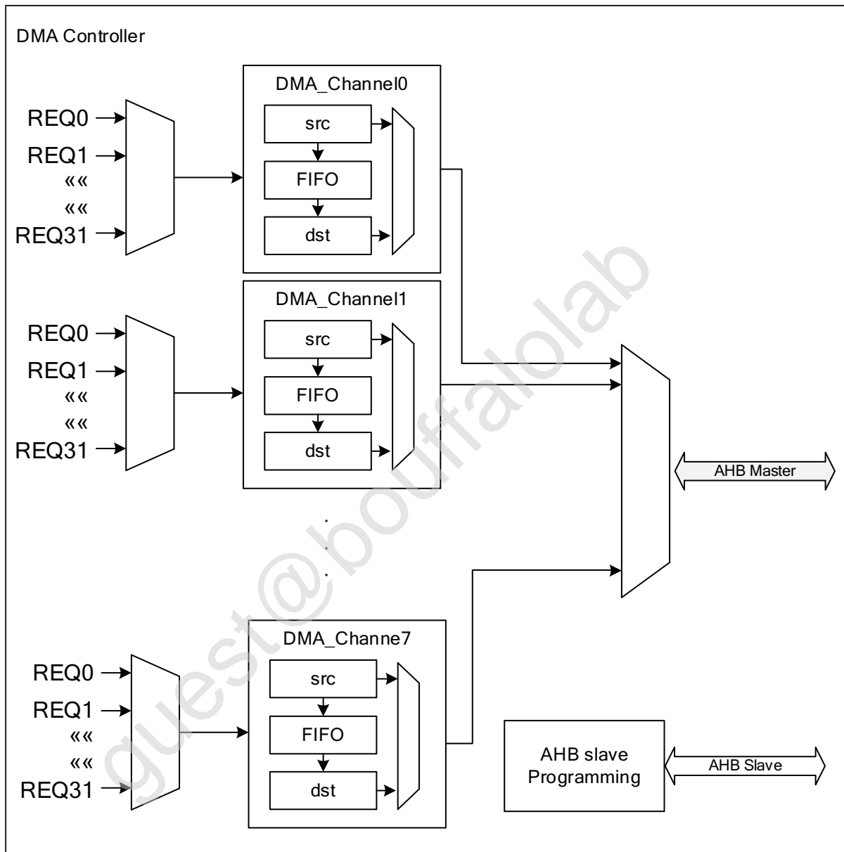
Fig. 6.1: DMA architecture
