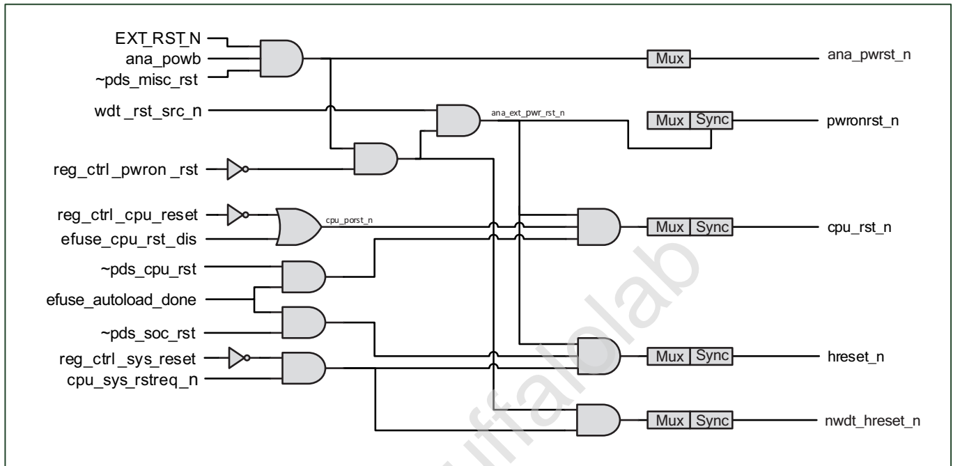
Fig. 2.1: Reset source
