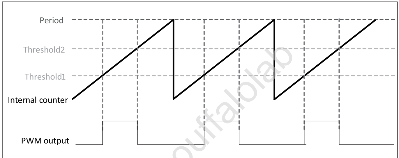
Fig. 12.1: PWM waveform
