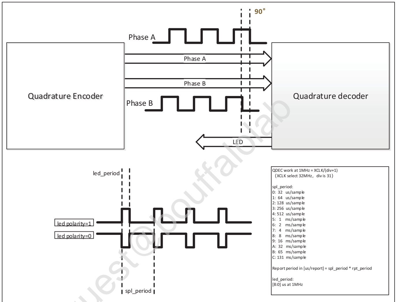
Fig. 14.1: QDEC functional block diagram
