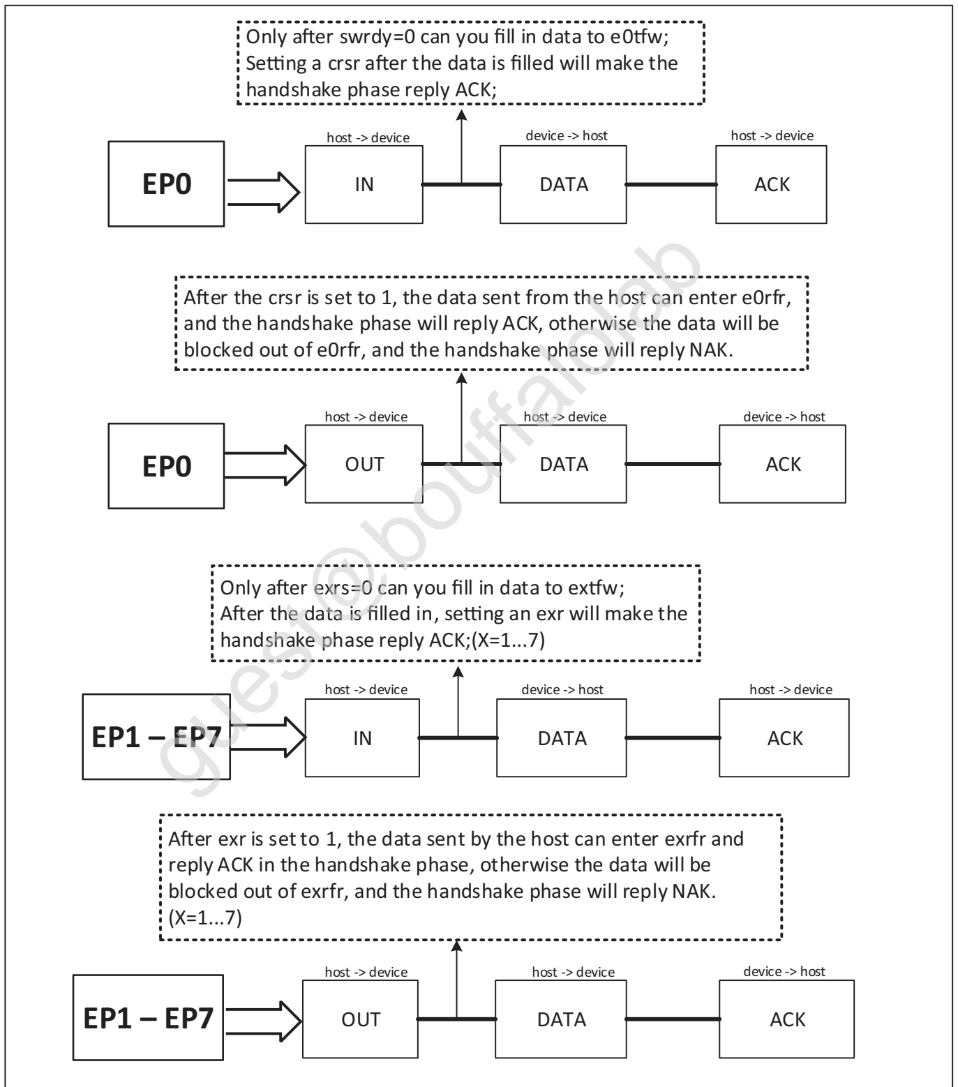
Fig. 18.2: USB communication method
