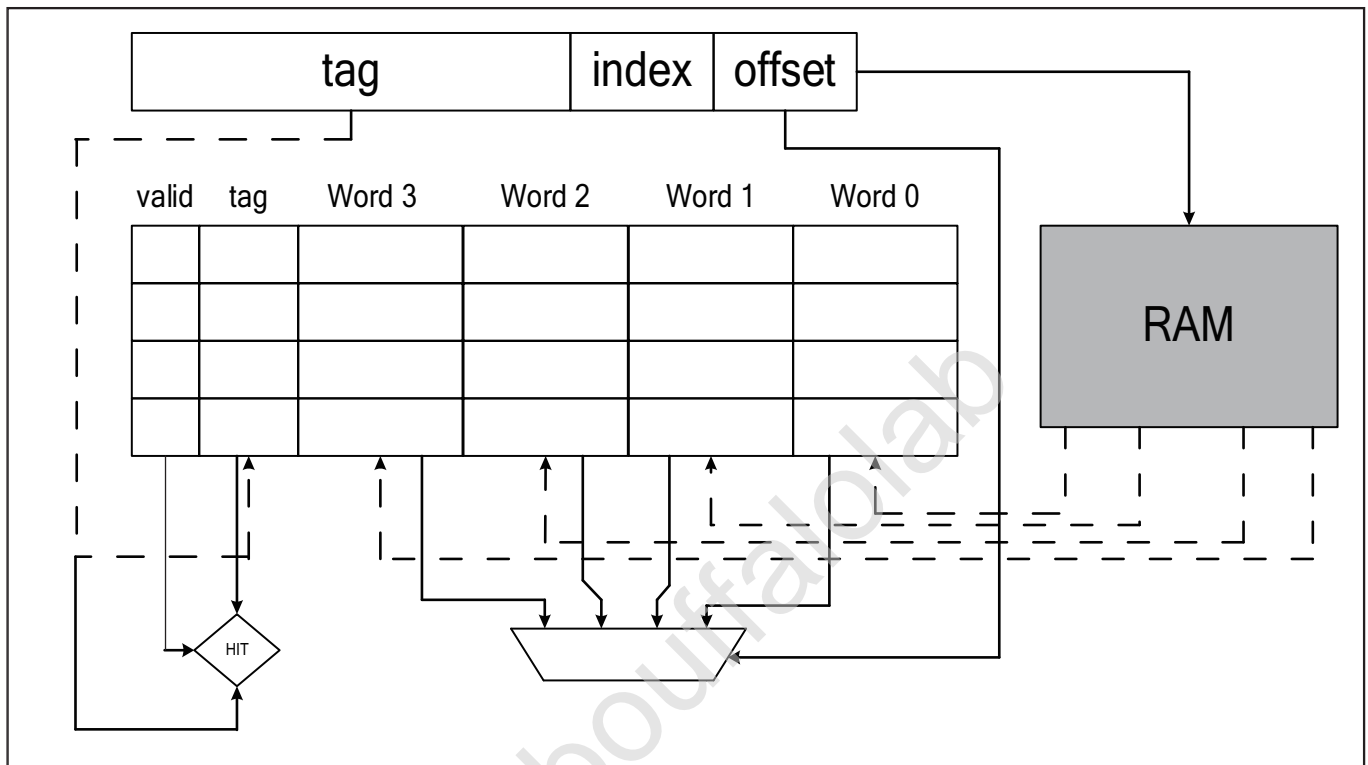
Fig. 7.2: Cache architecture
