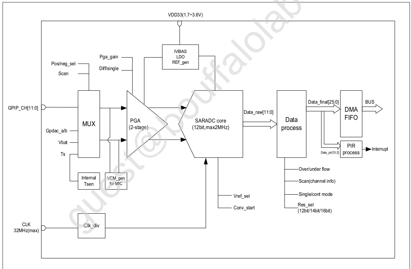
Fig. 4.1: ADC block diagram
