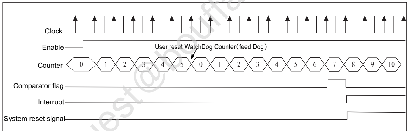
Fig. 13.4: Watchdog timing
