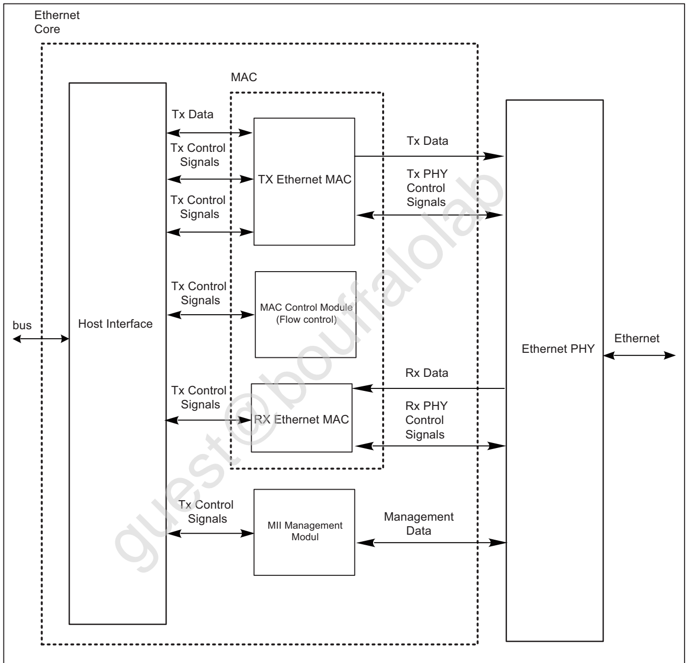
Fig. 17.1: EMAC architecture
