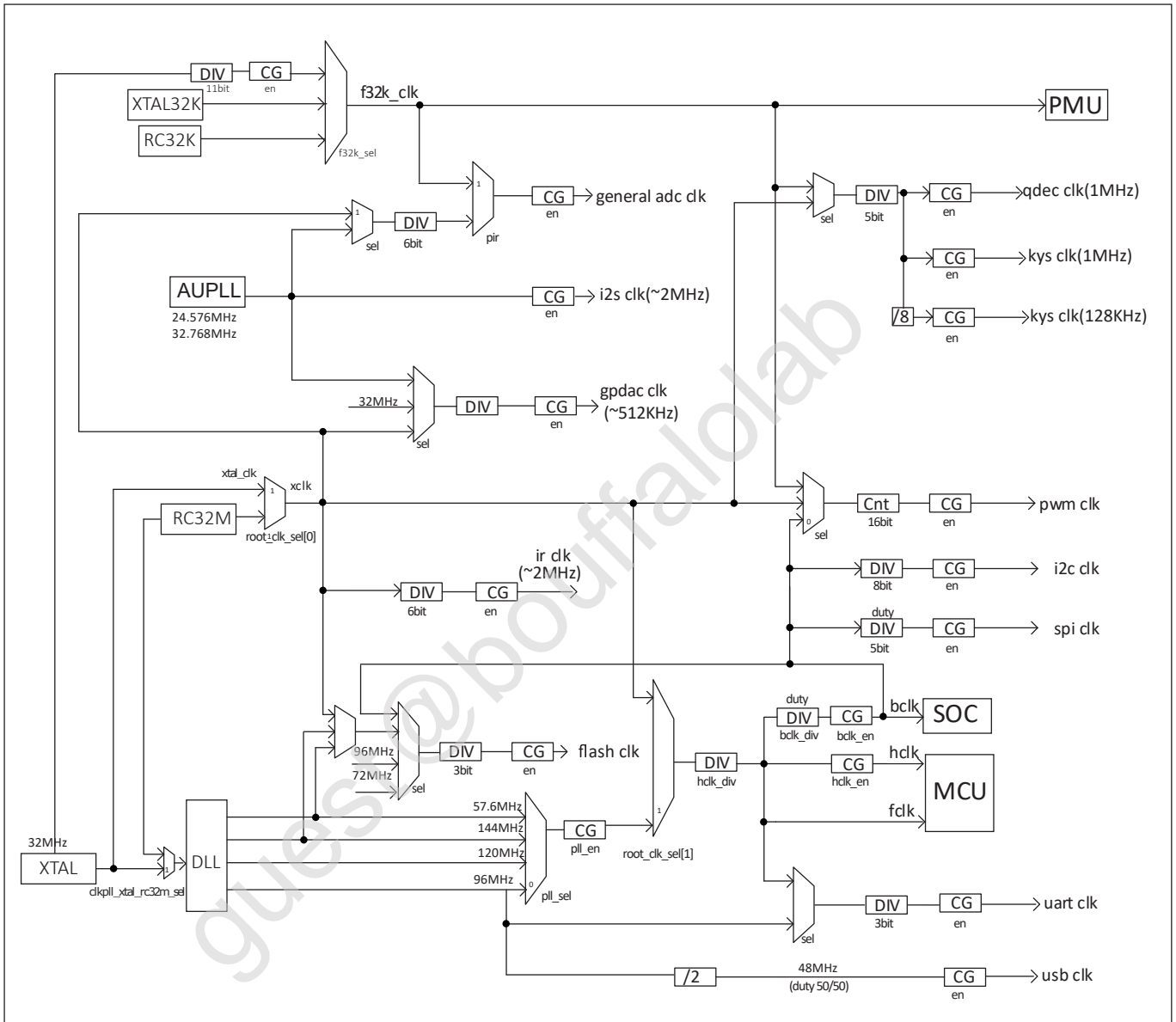
Fig. 2.2: Clock architecture
