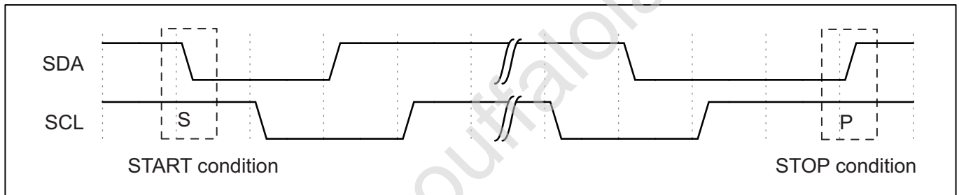
Fig. 11.1: I2C stop/start condition
